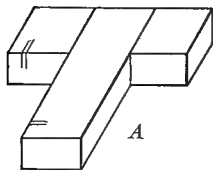
FIG. 50. Successive Steps in laying out and making a Middle Lap Joint
