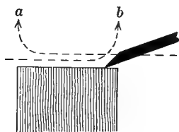
FIG. 27. Method of using Block Plane
