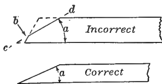
FIG. 29. Cutting Angle of Chisel
