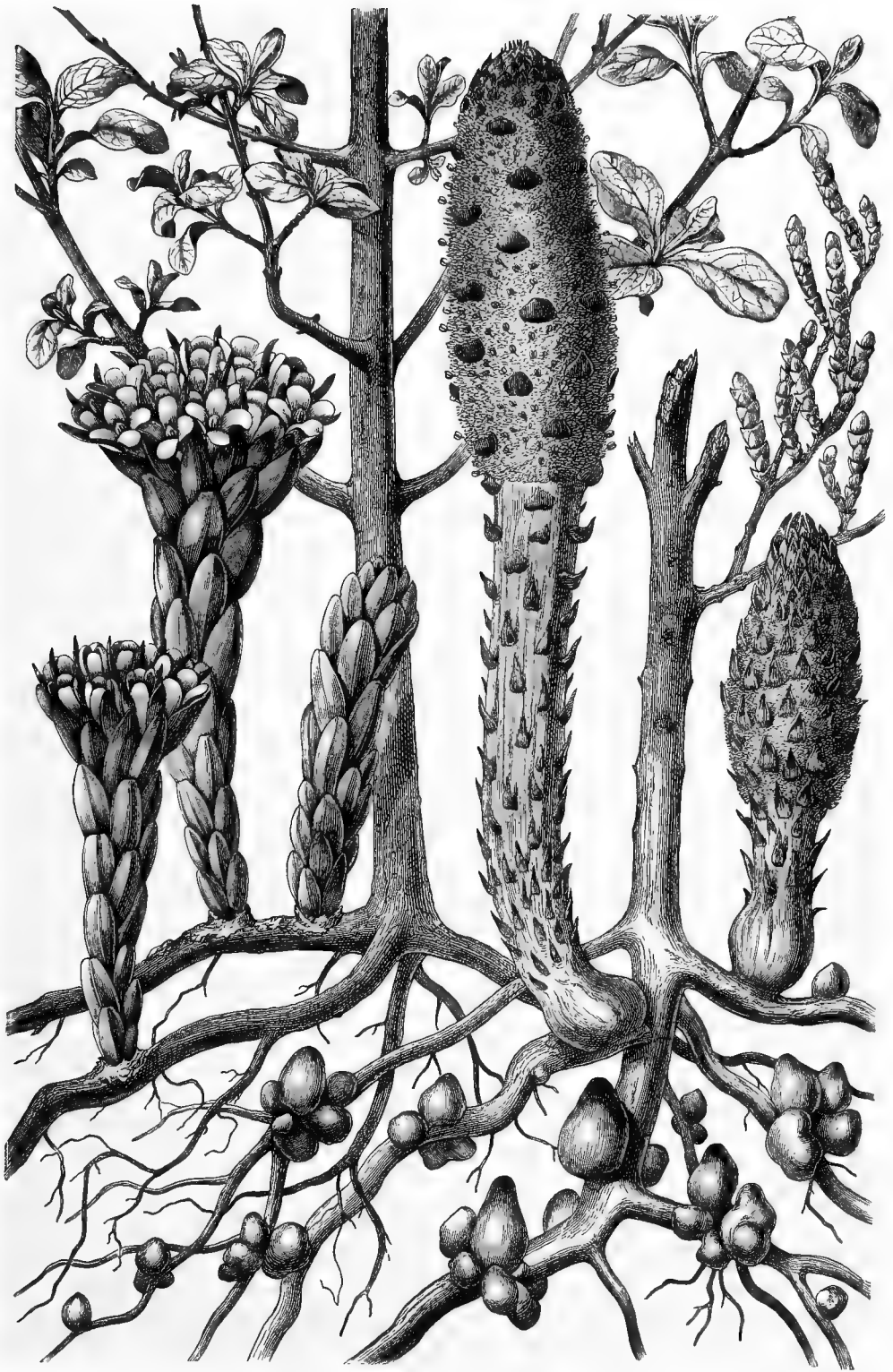
Fig. 42.— Cytinus Hypocistis on the left; Cynomorium coccineum on the right.
