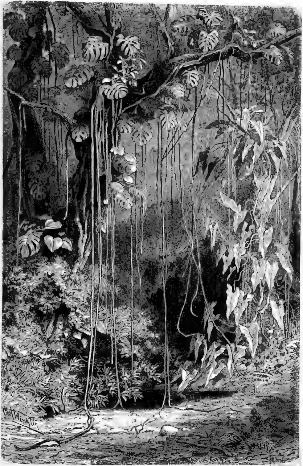
Fig. 96. — Aroids ( Philodendron pectusum and Philodendron Imbe ) with cord-like aerial roots.
