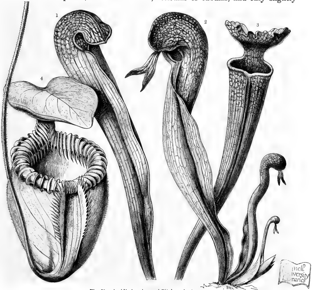
Fig. 21.—Ascidia-bearing and Pitcher-plants.
