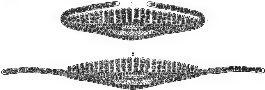
Fig. 89.—Folding of Moss-leaves.
