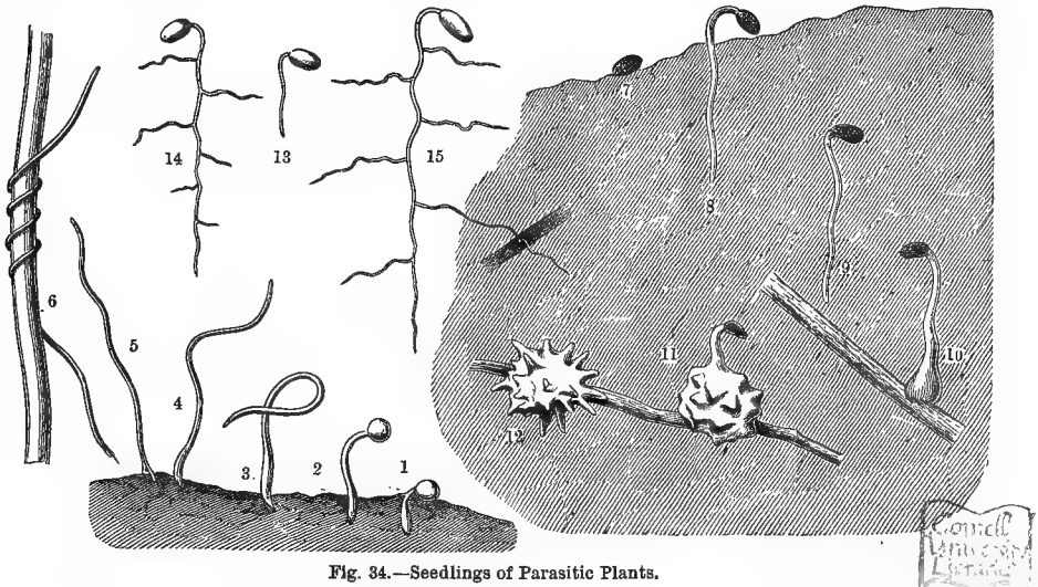
Fig. 34.—Seedlings of Parasitic Plants.
