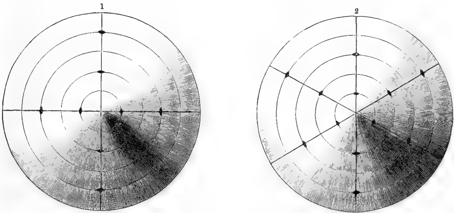
Fig. 98.—Plan of Whorled Phyllotaxis.
