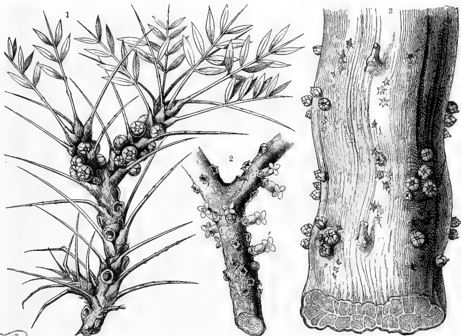
Fig. 43.—Rafflesiaceæ parasitic on trunks and branches.
