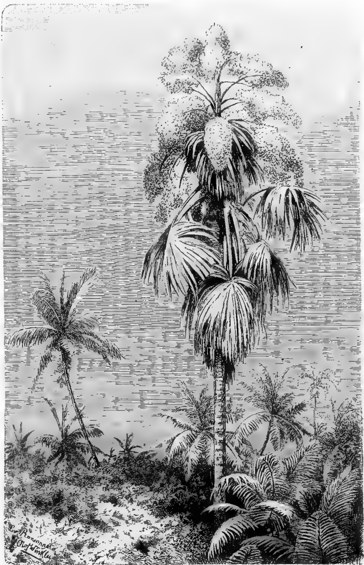
Fig. 63.— Corypha umbraculifera of Ceylon (after Ransonnet).
