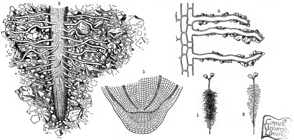
Fig. 12.—Absorptive Cells on Root of Penstemon .
