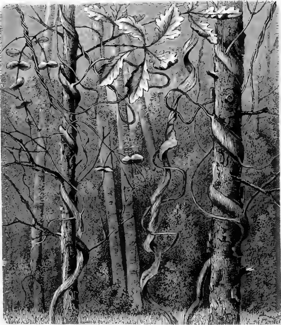
Fig. 31.— Lonicera ciliosa in South Carolina.
