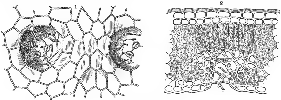
Fig. 68.—Stomata in Pit-like Depressions.
