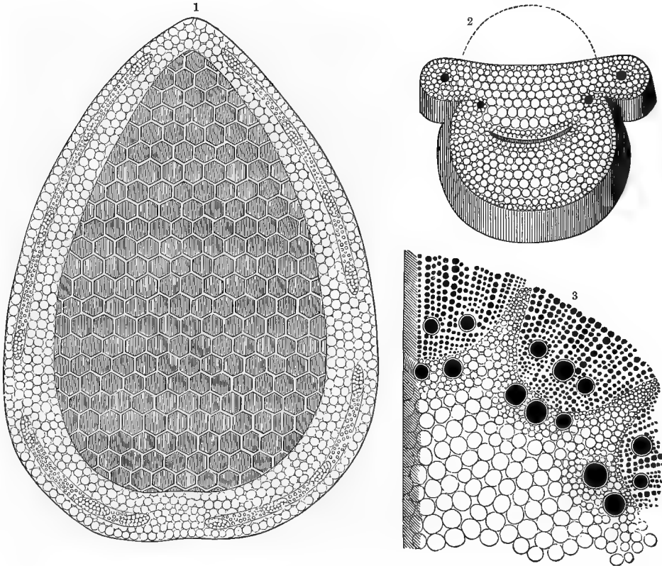
Fig. 4.—Vegetable Cells (from Grew's Anatomy of Plants ).
