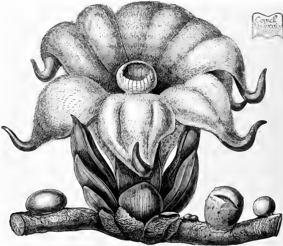
Fig. 44.—Parasitic Rafflesiaceæ ( Brugmansia Zipellii ) upon a Cissus -root.
