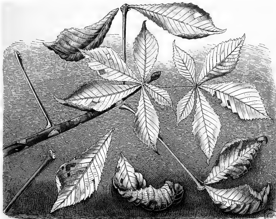
Fig. 93.—Leaf-fall of the Horse-chestnut ( Aesculus Hippocastanum ).
