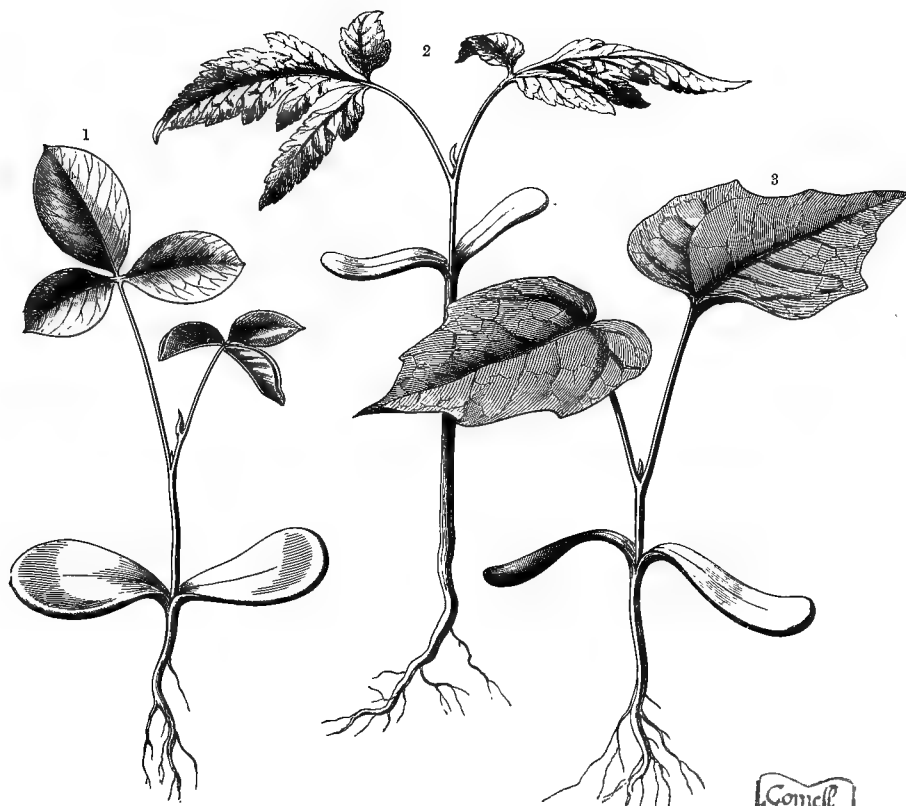
Fig. 1.—Seedlings with Cotyledons and Foliage-leaves.
