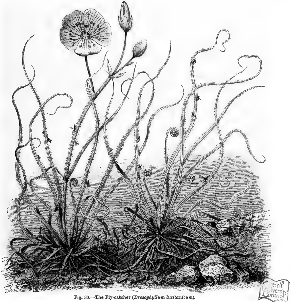
Fig. 30.—The Fly-catcher ( Drosophyllum lusitanicum ).
