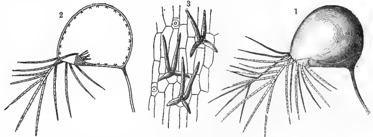
Fig. 18.—Traps of Utricularia neglecta .
