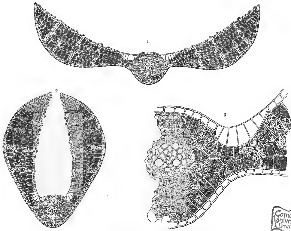
Fig. 85.—Folding of Grass-leaves.
