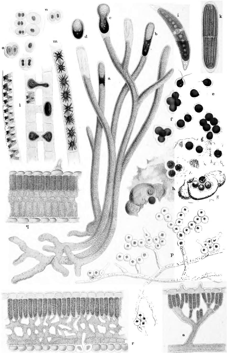
SWARM-SPORES AND ZYGOSPORES. FORMS OF CHLOROPHYLL-BODIES.
