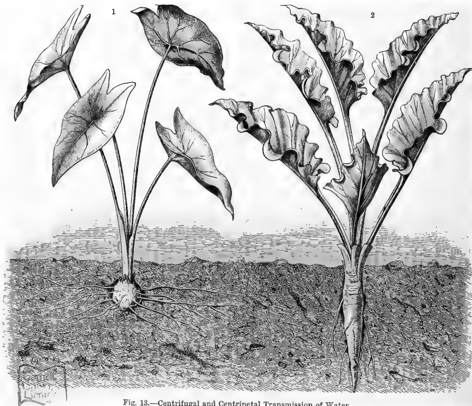
Fig. 13.—Centrifugal and Centripetal Transmission of Water.
