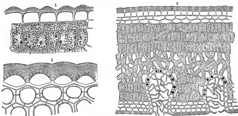
Fig. 73.—Thickened Stratified Cuticle.
