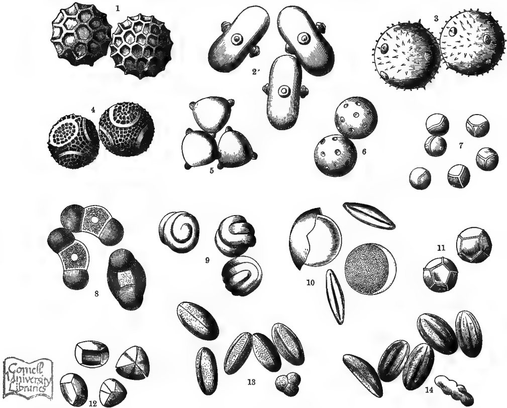
Fig. 217.—Pollen-grains.
