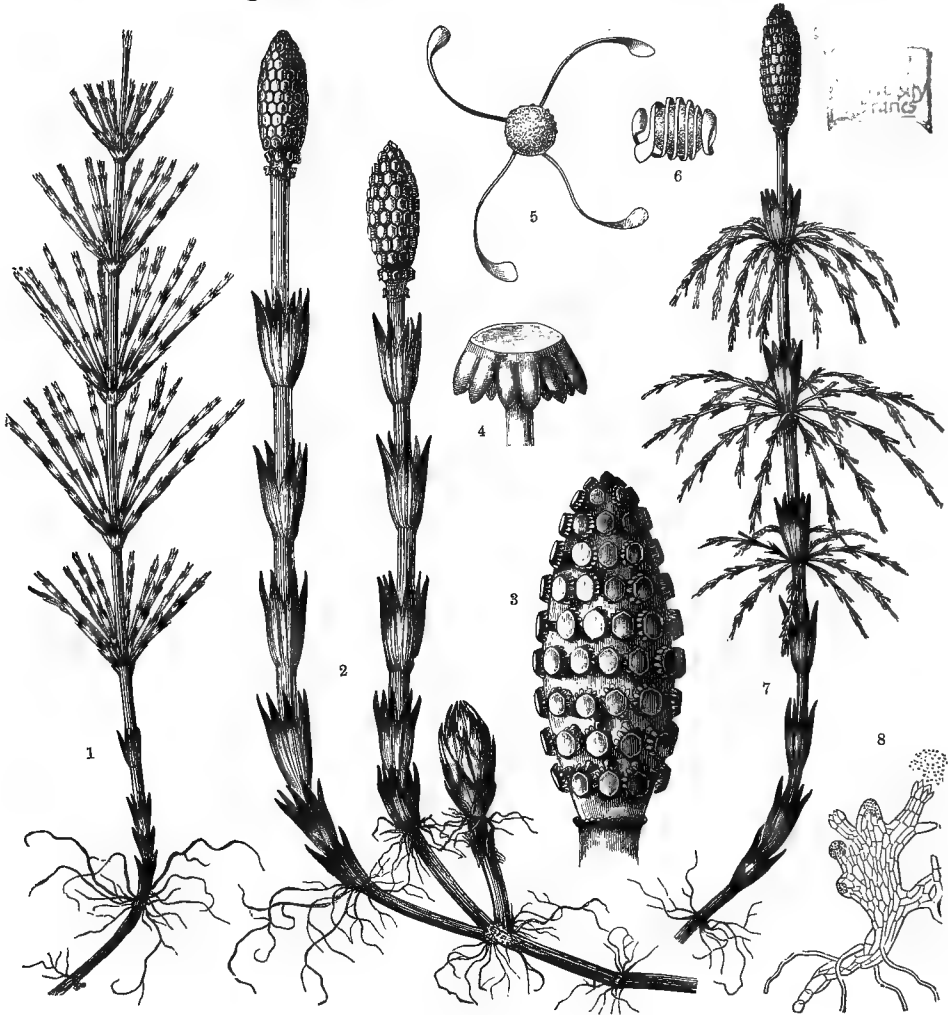
Fig. 190.—Horse-tails.
