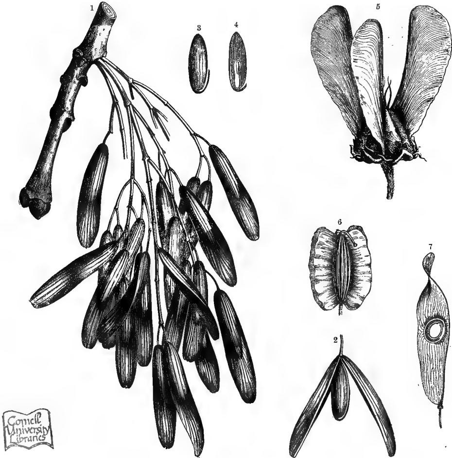
Fig. 323.—Winged Fruits.
