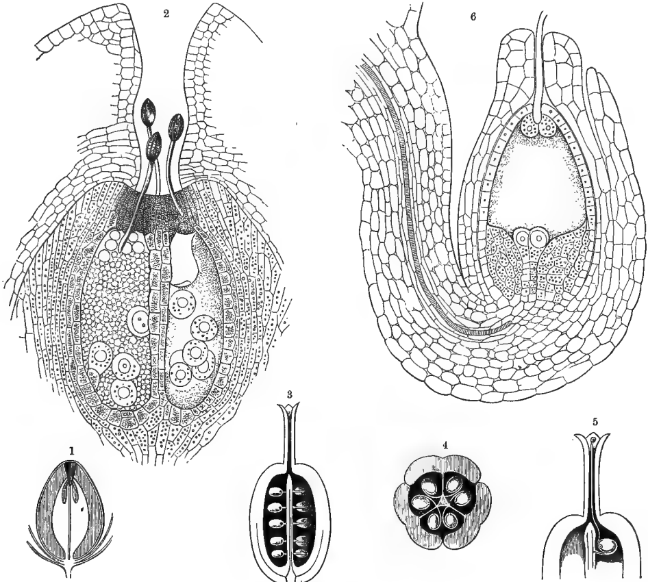
Fig. 315.—Fertilization.
