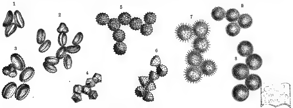
Fig. 218.—Pollen-grains.
