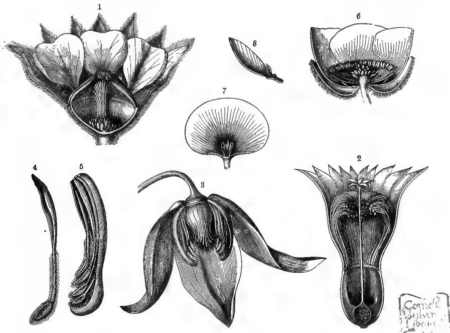
Fig. 246.—Nectaries.
