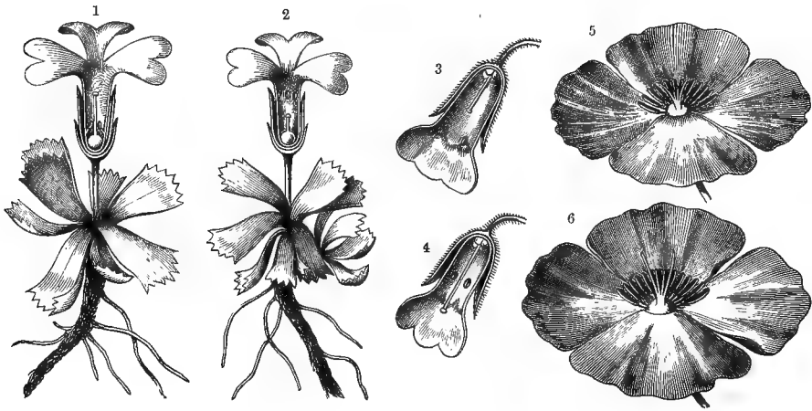
Fig. 288.—Heterostyled flowers.
