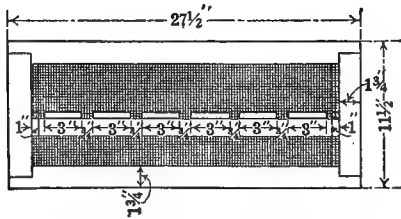
Mosquito trap, with details of construction.
