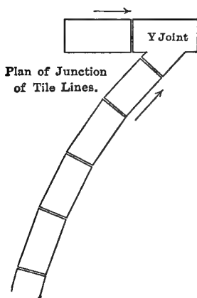
Plan and side view of junction of tile lines.
