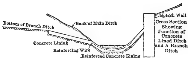
Junction of branch ditch with a lined ditch.
