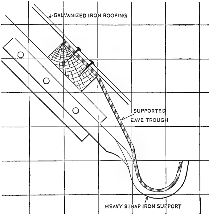
A firmly supported eave-trough.
