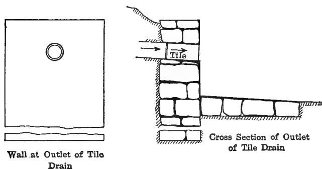
Detail of outlet of a tile drain.
