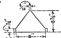
Wire Screen High Ridge Frame of White Pine
