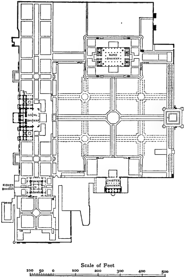
PLAN OF THE GARDEN-PALACE OF DEEG.
