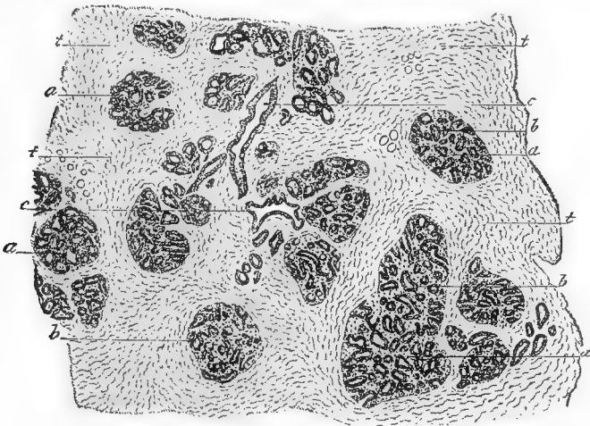
FIG. 162. —Section of mammary gland of woman. (From Sharpey Schafer, after de Sinéty.)
