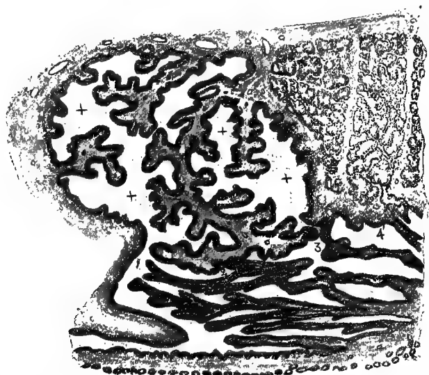
FIG. 125.—The labyrinth and the green border of the placenta of the dog at the fortieth day of pregnancy. To the right are two lobules of the angioplasmode which have reached the stage of complexity of the labyrinthine lamellæ: to the left is the green border, the cavities of which, normally filled with blood, are indicated by a cross. (From Duval's "Le Placenta des Carnassiers," Jour. de l'Anat. et de la Phys. , 1893.)
