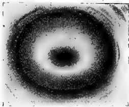
FIG. 160.—Virgin external os (human). (From Williams' Obstetrics . Appleton & Co.)
