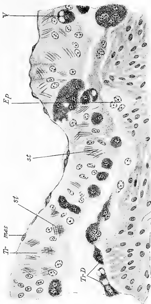
Fig. 121.—Absorption of "Stäbchen" by the trophoblast of the sheep. (Assheton.) mes. , Mesoblast; Tr. , trophoblast containing "Stäbchen" ( st ); Tr. D. , binucleate trophoblast cells; Ep , uterine epithelium undergoing absorption by the trophoblast; V , vacuolated cell.
