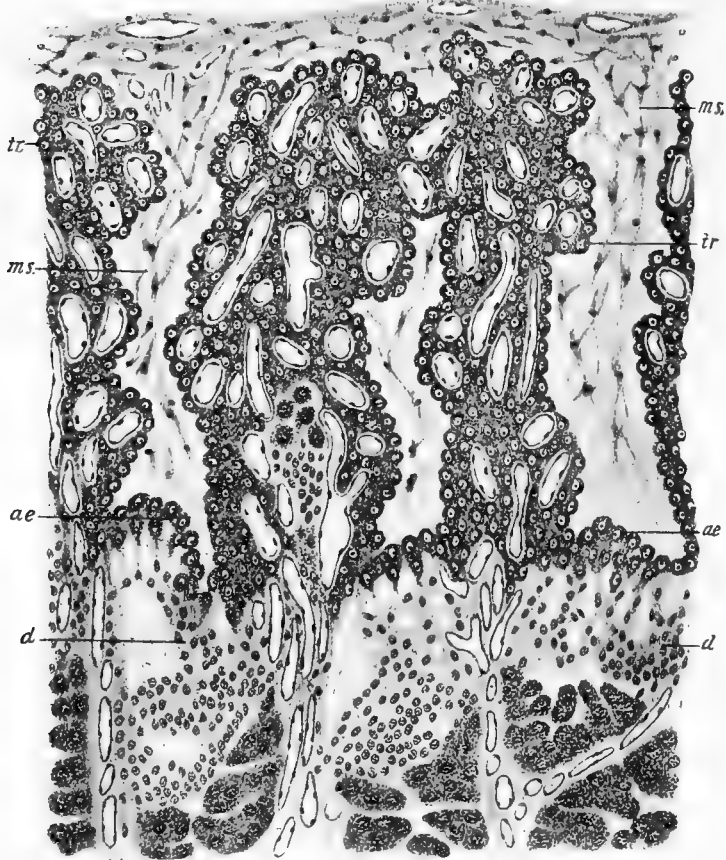
FIG. 124.—The angioplasmode of the dog at the thirtieth day of pregnancy. (From Duval's "Le Placenta des Carnassiers," Journ. de l'Anat. et de la Phys. , 1893.)
