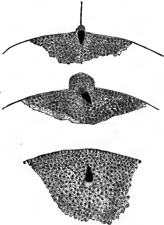
FIG. 56. — Successive stages in the fertilisation of an ovum of Echinus esculentus , showing the entrance of the spermatozoon. (From Bryce.)
