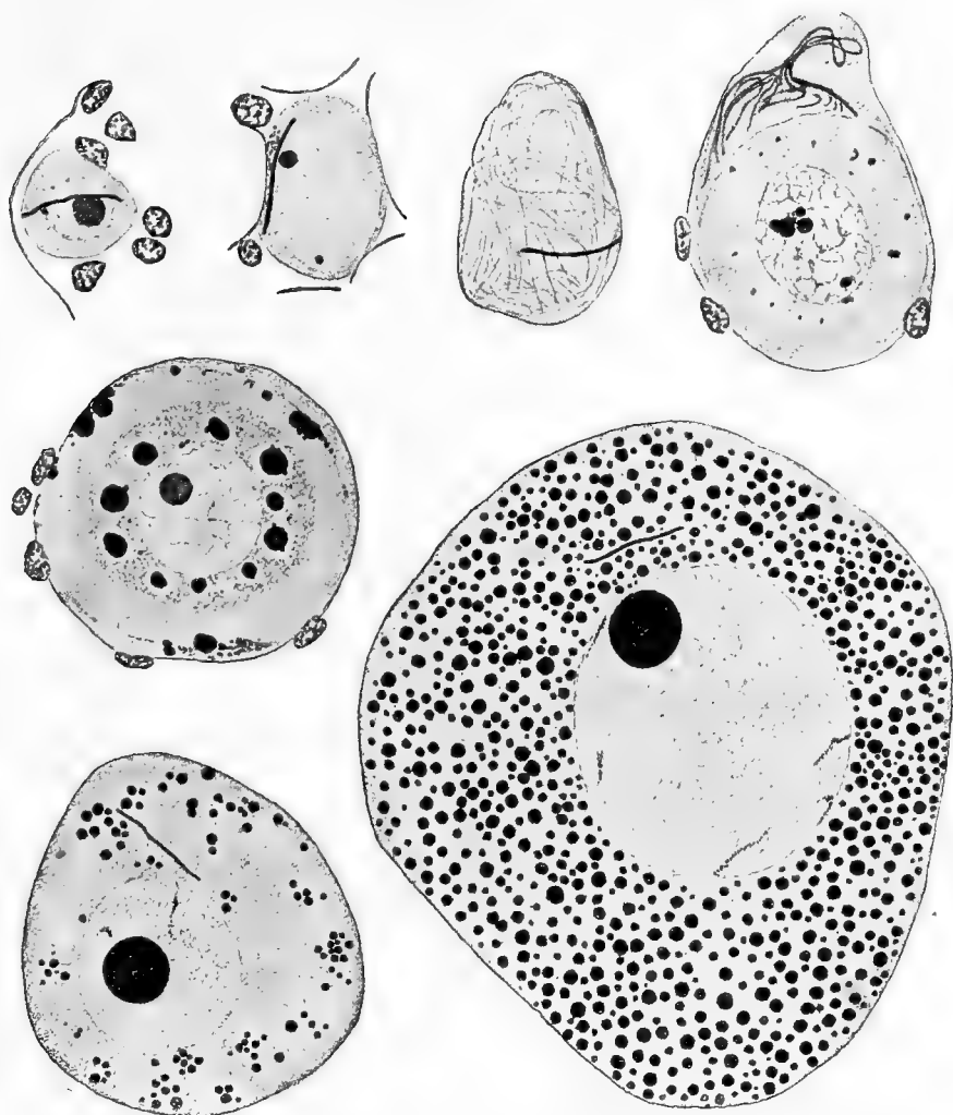
FIG. 60.—The insemination of the eggs of Saccocirrus while these are undergoing growth in the ovarian tissue. The long black rod-like body in the cytoplasm of the primitive oocytes is the spermatozoon. It will be seen that the ovum develops from a very early stage with the spermatozoon in its cytoplasm, actual fusion of sperm and female pronucleus only taking place after the eggs are laid and have undergone meiosis. (From Buchner's Praktikum der Zellenlehre , Bd. i., Borntraeger.)
