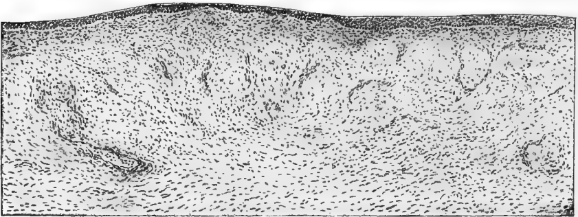
FIG. 185.—Section through vaginal mucous membrane of woman of sixty-one. (From Sellheim.)
