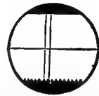
Field of large filar micrometers showing cross hairs and recording comb.
