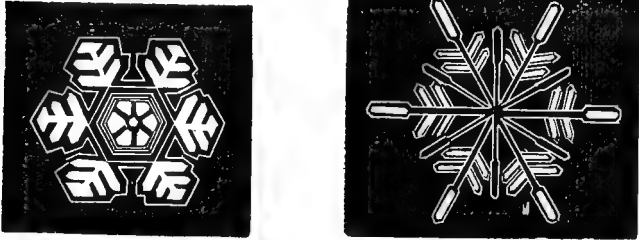
fig. 84. Snow Crystals.
