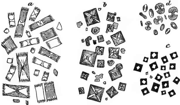
fig. 80. Urinary Salts.
