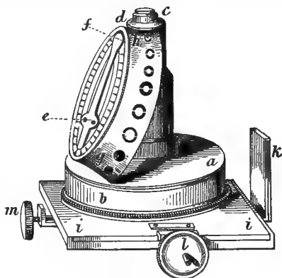
fig. 39. Gillett's Condenser.
