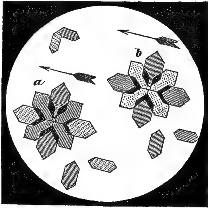
fig. 81. In this figure the heraldic lines are adopted to denote colour. The dotted parts indicate yellow , the straight lines red , the horizontal lines blue , and the diagonal, or oblique lines, green . The arrows show the plane of the tourmaline, a , blue stage; b , red stage of selenite employed.
