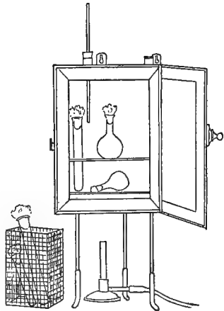
FIG. 398A.—A hot-air steriliser.— From Muir and Ritchie.
