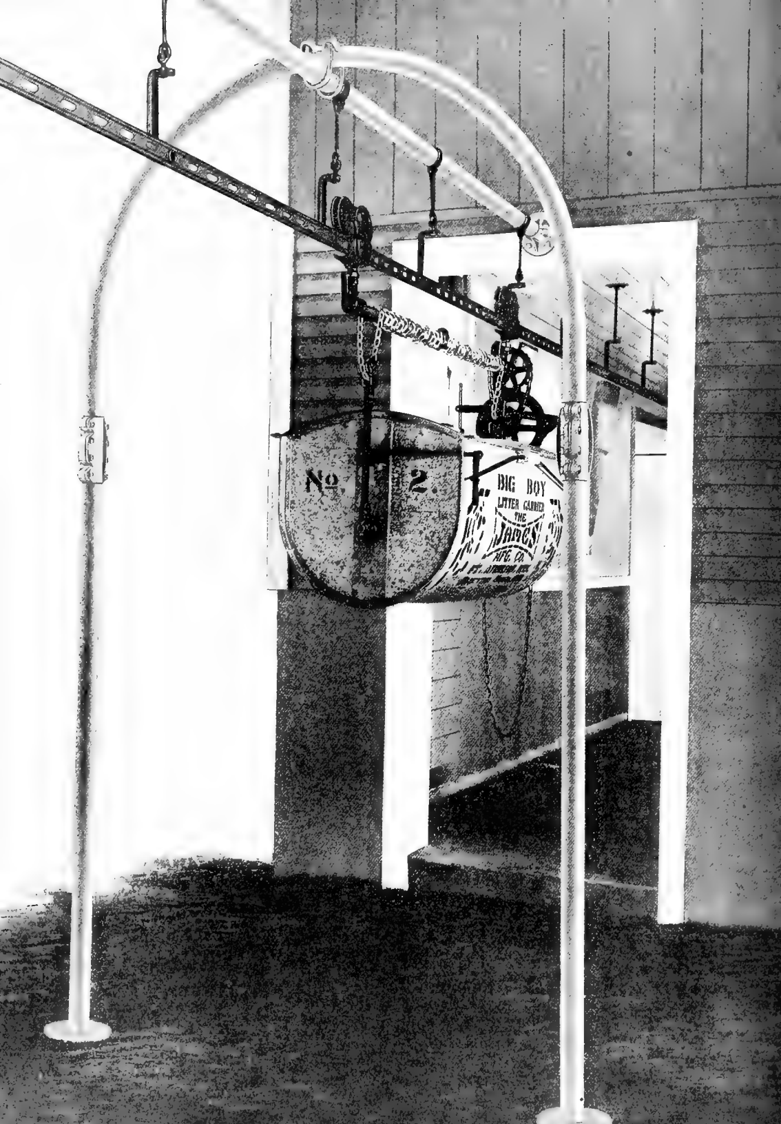
James Carrier Outside Support.
