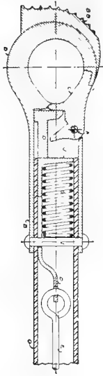
Cross Section of Lock Hook
