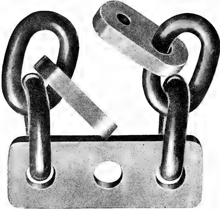
Actual size of James Double Chain Hanger Links. Links 1\frac{1}{8} " long inside \frac{3}{8} " diameter.
