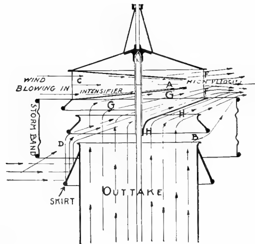
Fig. 10 James Revolving Hood Ventilator
