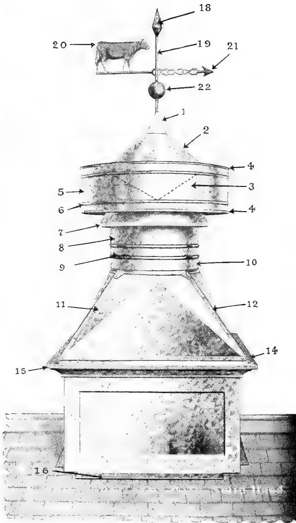
Fig. 4 Sizes 24 and 30 inch Weight crated Ventilator No. 3, 24 in. — 206 lbs. Ventilator No. 4, 30 in.— 320 lbs.
