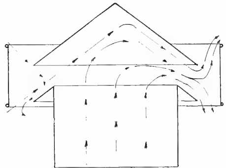
Fig. 8 Metal Cupola with Storm Band
