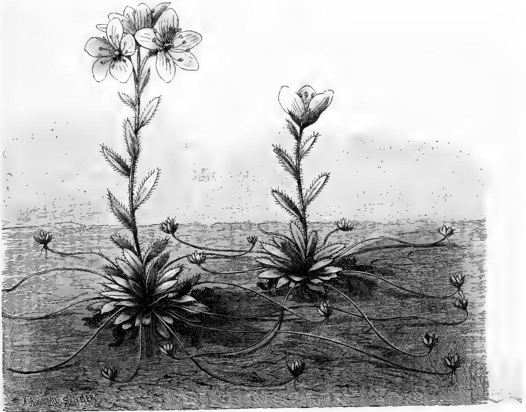
Fig. 446.—Formation of a clustered colony by means of aerial runners in Saxifraga flagellaris .
