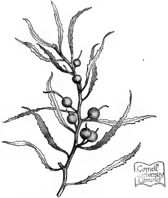
Fig. 378.—A branch of the Gulf-weed, Sargassum bacciferum , with leaves and air-sacs.
