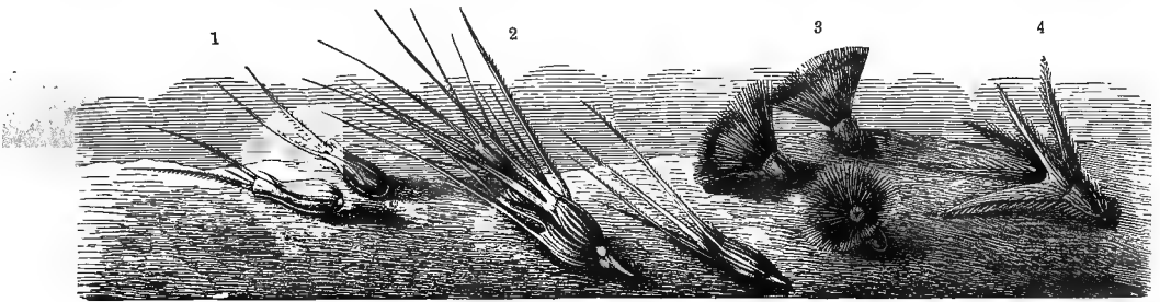
Fig. 461.—Creeping and hopping fruits.
