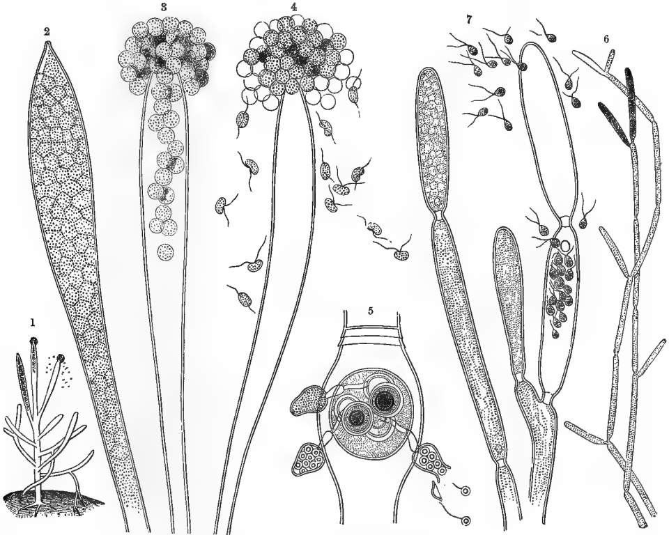
Fig. 380.—Swarm-spores in Saprolegniaceæ and Chytridiaceæ.
