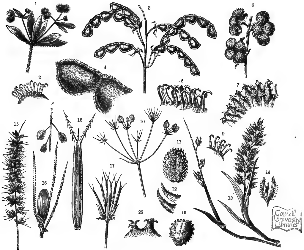
Fig. 477.—Fruits furnished with hooks.
