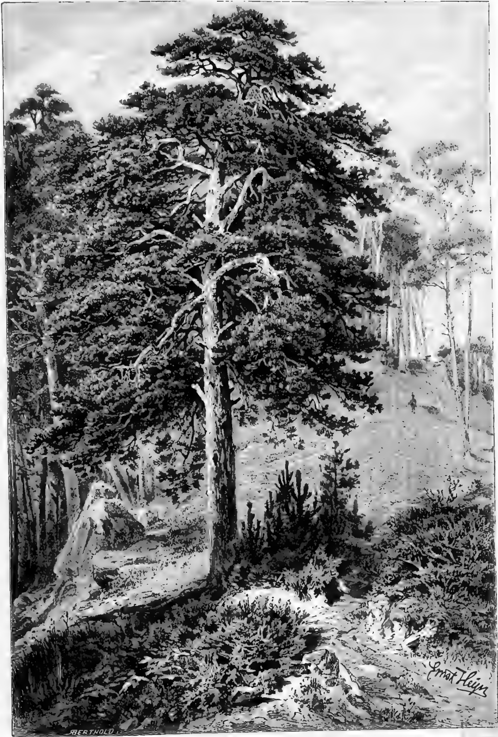
Fig. 400.—The Scotch Pine ( Pinus sylvestris ).
