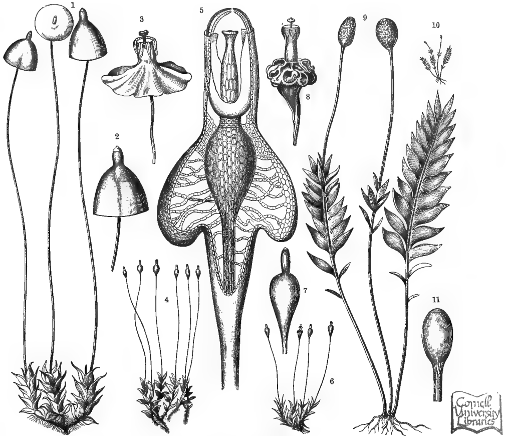
Fig. 399.—Spore-capsules of Mosses.
