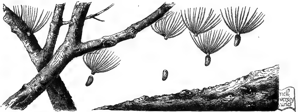
Fig. 474.—Dispersion of fruits and seeds by the wind. Fruits of a Thistle ( Cirsium nemorale ) floating in the air and becoming detached from their parachutes and dropping to the ground whenever they encounter an obstacle in the course of their flight.
