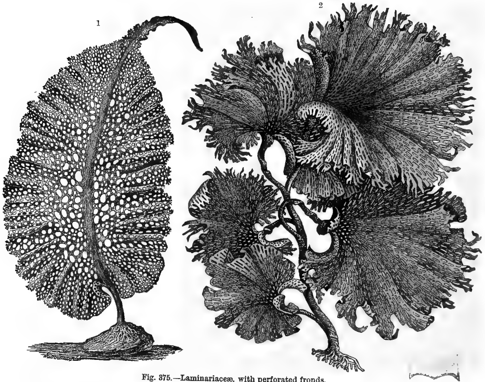
Fig. 375.—Laminariaceae, with perforated fronds.
