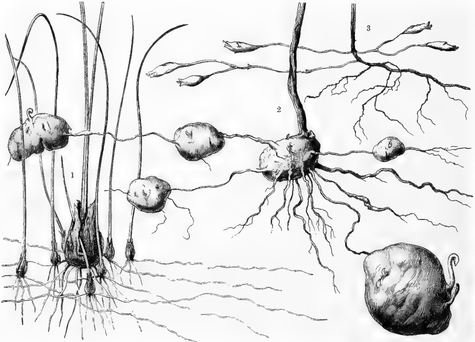
Fig. 444.—Plants with tubers and bulbs whose mode of growth leads to the formation of colonies arranged in lines and clusters. 1 Muscari racemosum . 2 Thladiantha dubia . 3 Circaea alpina .
