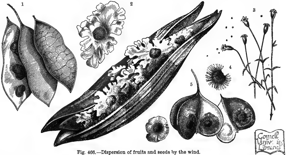
Fig. 466.—Dispersion of fruits and seeds by the wind.
