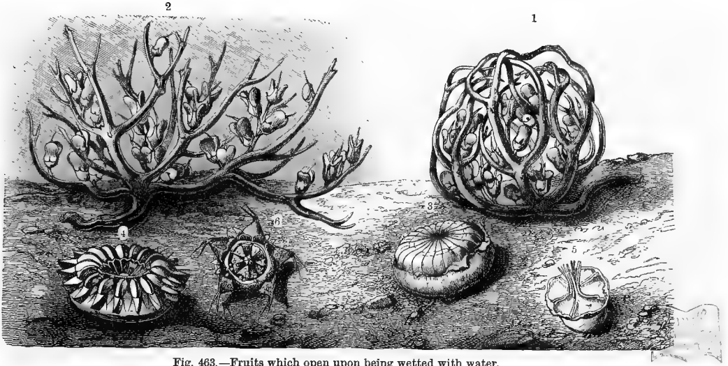
Fig. 463.—Fruits which open upon being wetted with water.
