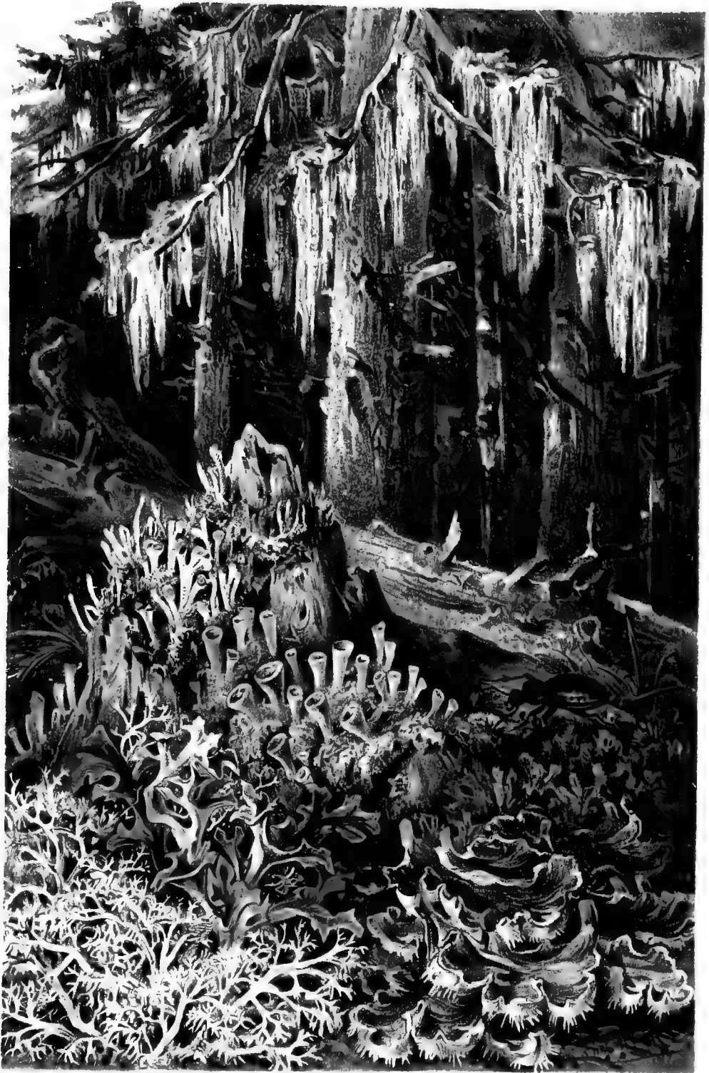
FRONDOSE AND FRUTICOSE LICHENS.
