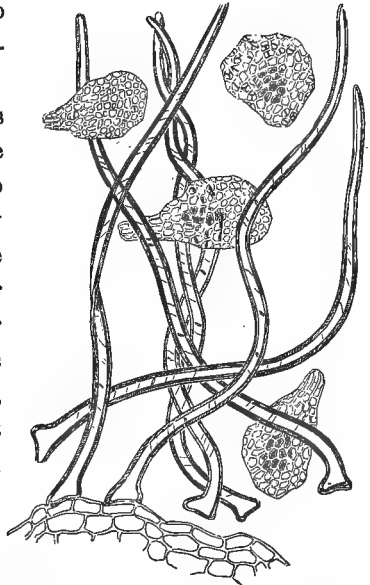
Fig. 478.—Seeds of the Orchid Vanda teres , which are moved from the interior to the surface of the capsule by hygroscopic hair-like cells, and are thus exposed to the wind; \times 100 .
