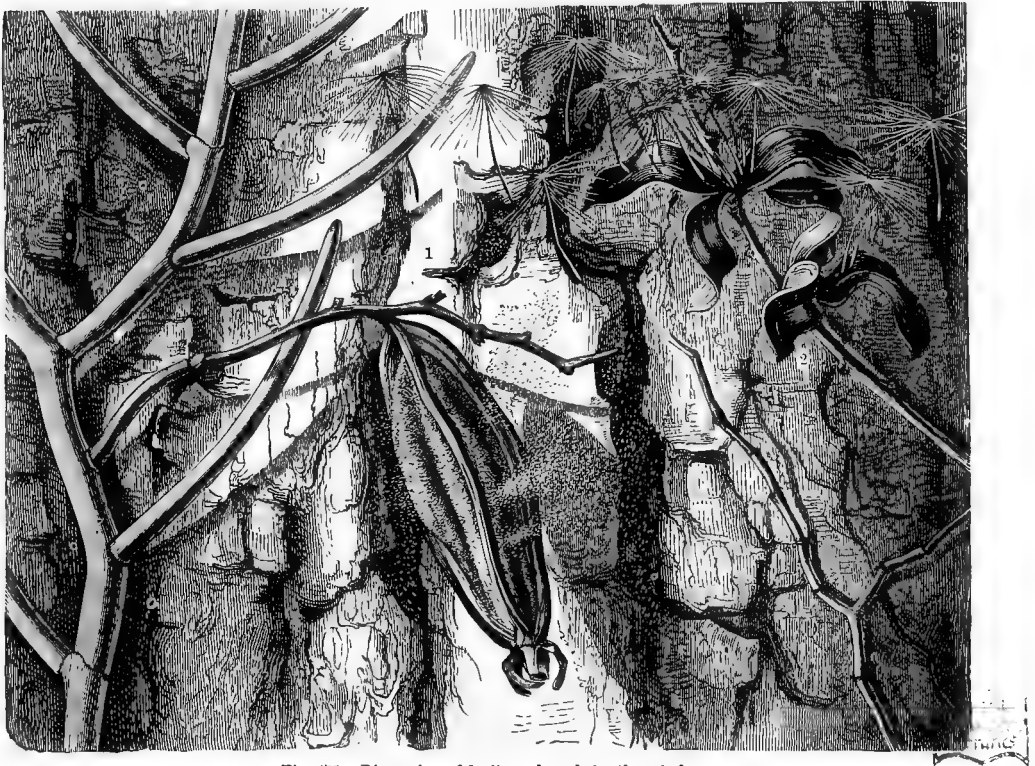
Fig. 475.—Dispersion of fruits and seeds by the wind.
