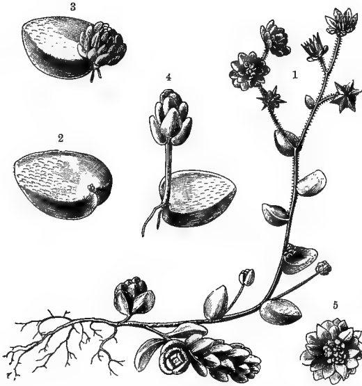
Fig. 454.—The formation of offshoots in Sedum dasyphyllum .
