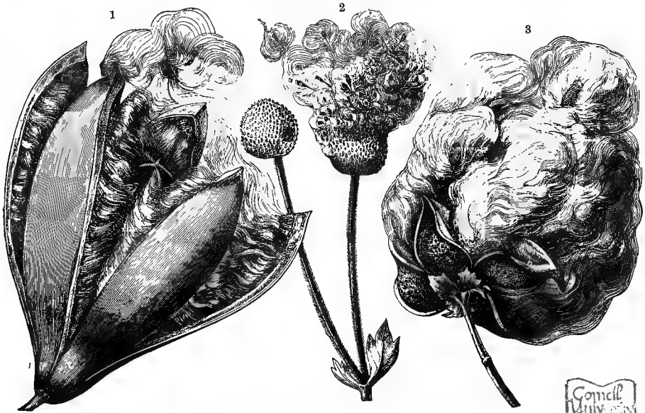
Fig. 470.—Dispersion of fruits and seeds by the wind.
