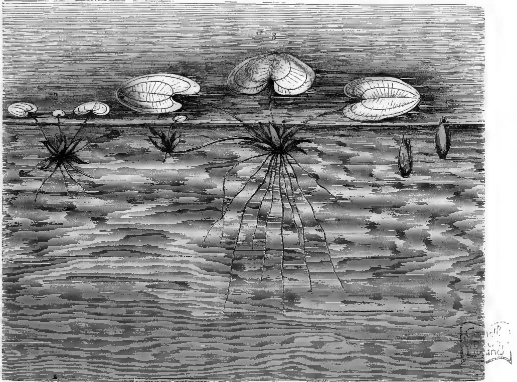
Fig. 448.—Frogbit ( Hydrocharis Morsus-ranæ ). 1 Winter buds rising to the surface in spring. 2 Young floating plants which have developed from such buds. 3 Older floating plants.
