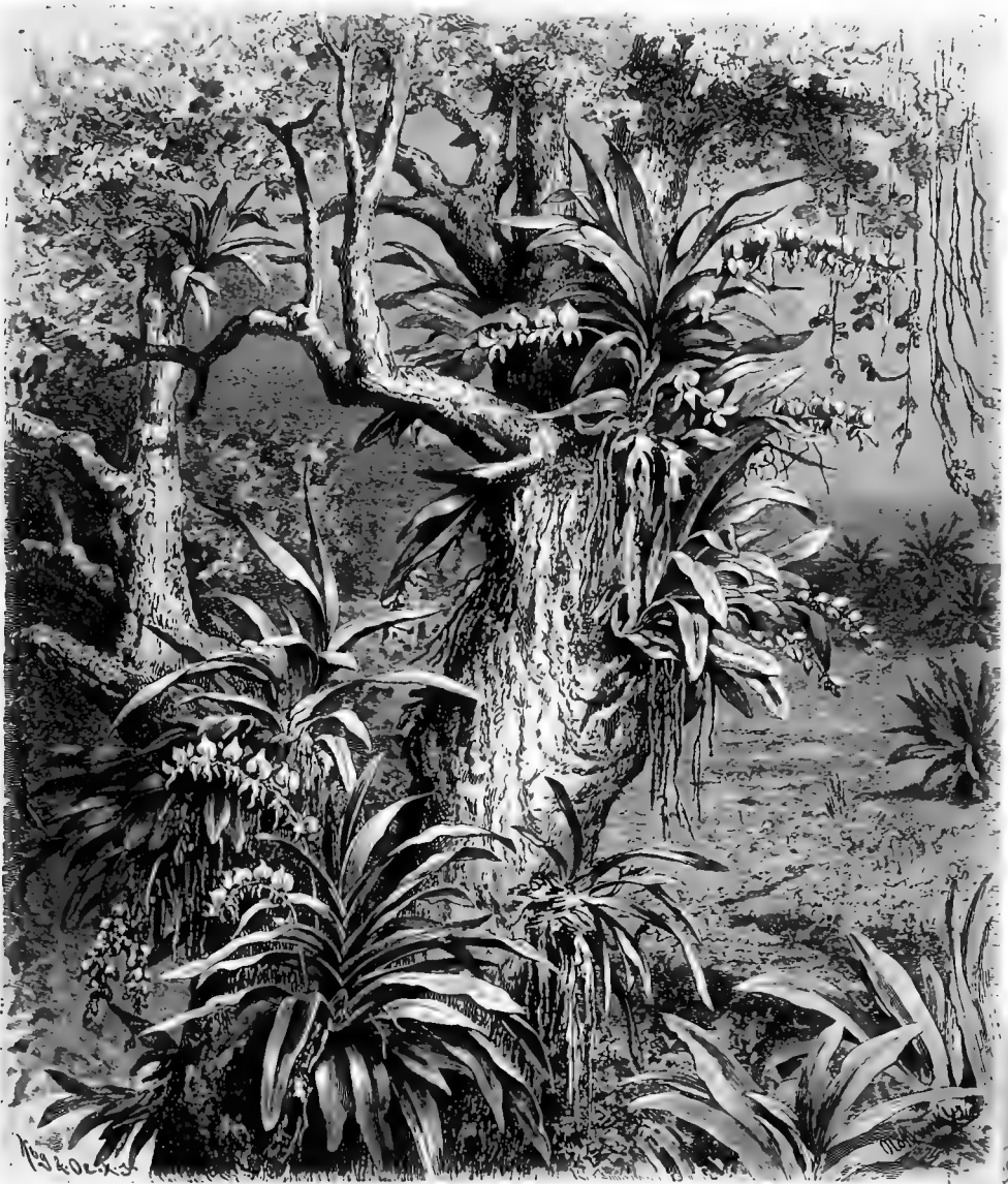
Fig. 418. — Angraecum eburneum epiphytic on a tree-trunk (Madagascar).
