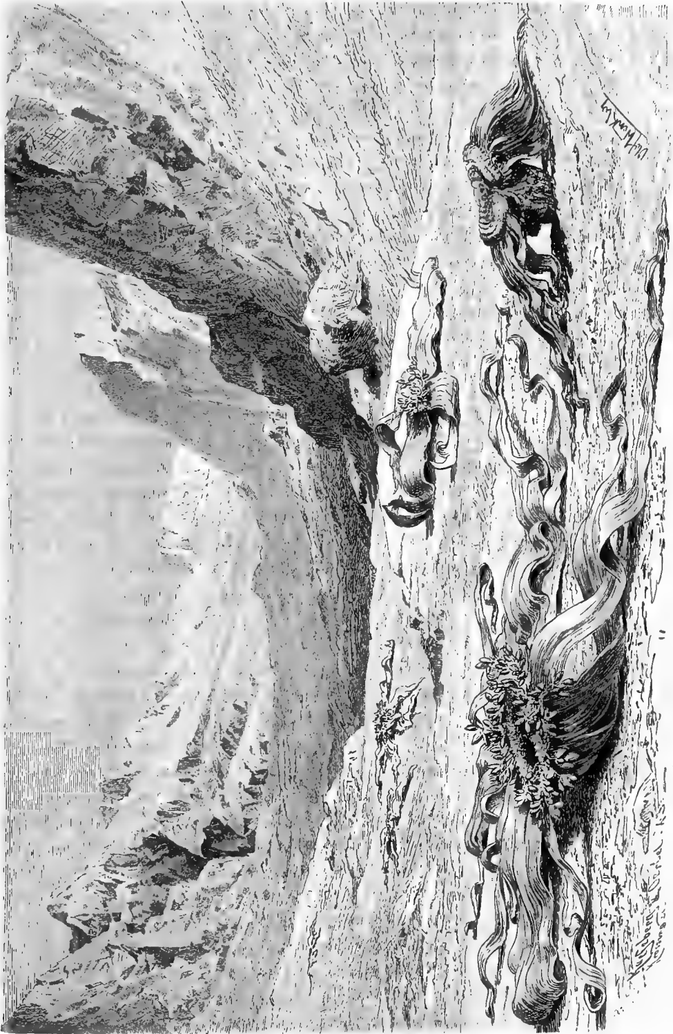
Fig. 411. — Wetitschia mirabilis in its natural surroundings (from a sketch by its discoverer).
