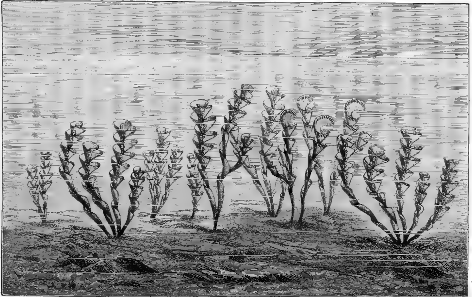
Fig. 366.— Riella helicophylla growing under water. Enlarged.
