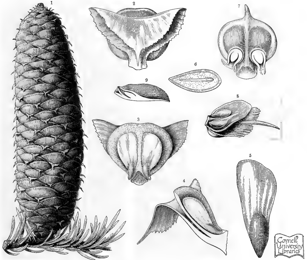
Fig. 407.—Female Cone and Scales in Abietineæ.
