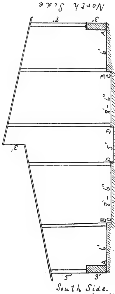
Cross-section of piggery, showing contour of floor, shape of roof, and supports for same.
