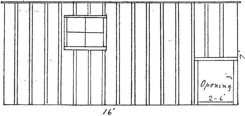
16' Front view of portable pen.
