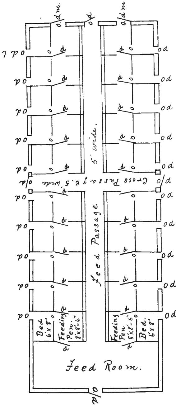
PLAN OF PIGGERY. Explanations:—o. Openings 2½ feet wide between bed and feeding pen. d. Doors 4 feet wide in partitions, which swing back and close openings at o. o. d. Doors leading outside. o. d. m. Doors for taking out manure, or taking in bedding. Pens are uniform size throughout. Dimensions of pens include partitions.
