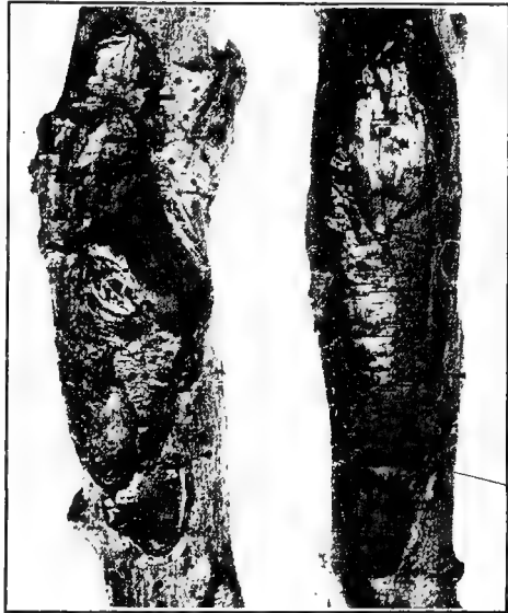
FIG. 6. — Bitter-rot cankers.
