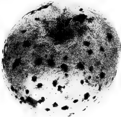
FIG. 24. — Apple fruit-spot.
