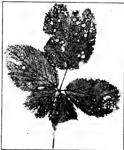
FIG. 46. — Blackberry leaf-spot.
