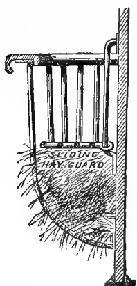
Fig. 111.—Section of sliding hay-guard seen in Fig. 110 (Musgrave).
