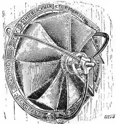
Fig. 25.—Blackman Air-Propeller.
