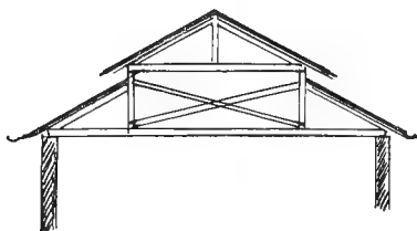
Fig. 85.—Open Roof.
