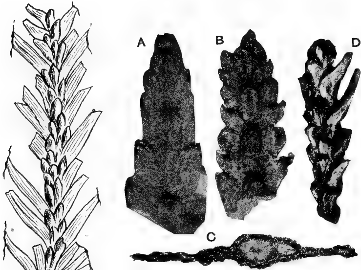
FIG. 806. A—C, Androvettia statenensis . D, Geinitzia Reichenbachii . (A, B, \times 6 ; C, \times 7 ; D, \times 7 ; after Hollick and Jeffrey.)
