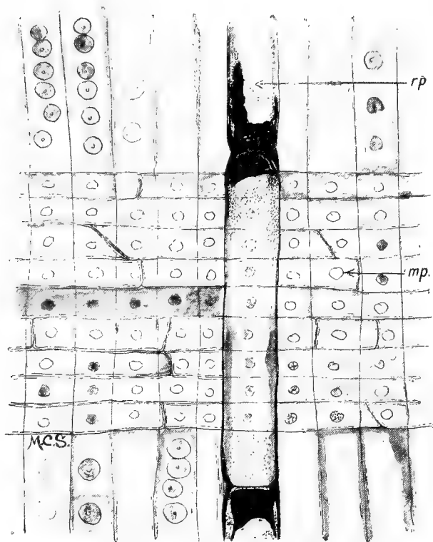
FIG. 717. Cupressinoxylon Hortii . Radial section showing the pits of the medullary rays, mp ; the pits on the tracheids, and the wood-parenchyma, rp . (After Stopes.)
