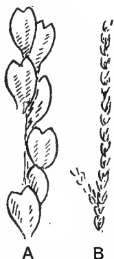
FIG. 809. Schizolepidella gracilis . (After Halle; A, enlarged; B, nat. size.)
