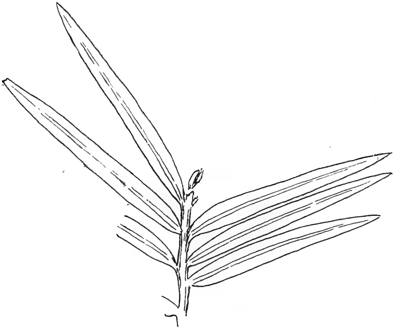
FIG. 795. Podocarpites Campbellei . (After Gardner; nat. size.)
