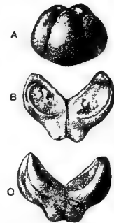
FIG. 761. Callitrites curta . A, cone of five valves. B, C, two views of a section of a four-valved cone. (British Museum, drawn from specimens described by Gardner; nat. size.)
