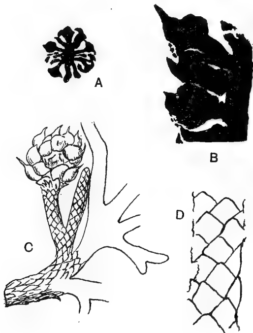
FIG. 753. A, B, D, Athrotaxites Ungerii . C, Athrotaxites lycopodioides . (A, B, D, after Halle; A, nat. size. C, after Saporta; nat. size.)
