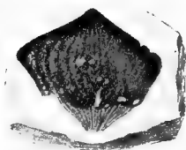
FIG. 733. Dammarites borealis . Cone-scale from Igdlökungnak, West Greenland. (Stockholm Museum; nat. size.)
