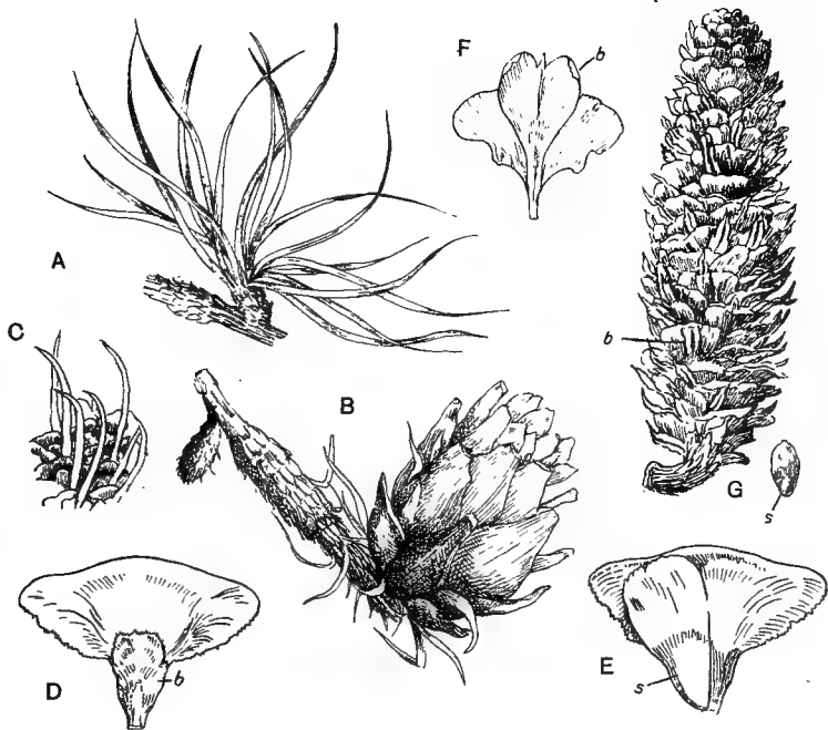
FIG. 705. A, B, Short shoot and cone of Pseudolarix Kaempferi . C, Abies bracteata , showing the long bract-scales. D, E, Abies concolor , cone-scale; b, bract-scale; s, seed. F, Abies Fraseri , cone-scale; b, bract-scale. G, Larix Griffithi ; b, bract scale; s, seed. (C—F, from the Gardeners' Chronicle .) M. S.
