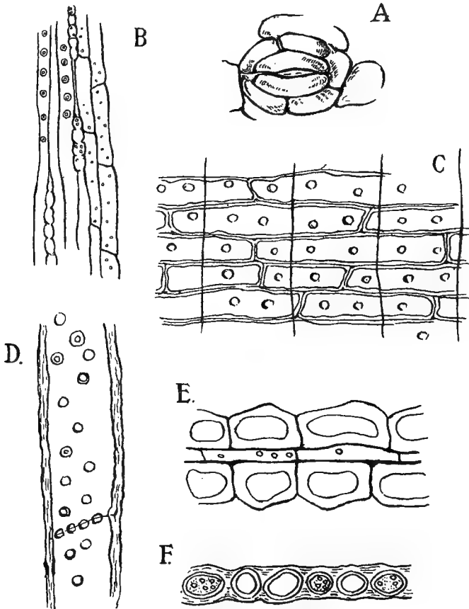
FIG. 724. A, Brachyphyllum eathiense ; stoma. B—F, Cedroxylon Hornei . (After Seward and Bancroft.)
