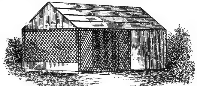
FIG. 4.—HOUSE 24x36 INCHES. COVERED RUN FOR CHICKS; SEPARATE APARTMENT FOR HEN; DROP DOOR IN FRONT; APARTMENT FOR HEN 12x24.
