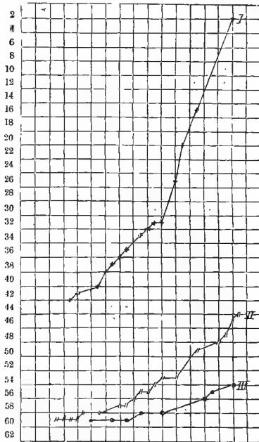
FIG. 27.—The mean thermal curves detected by Rossbach for the contractile vesicle of Infusoria. I. For Euplote Charon . II. For Syltonychia pustulata . III. For Chilodon cucullulus . The animals are shown in fig. 28.
