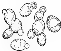
FIG. 275.—YEAST PLANTS.
