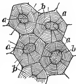
FIG. 84. — GRIT CELLS.
