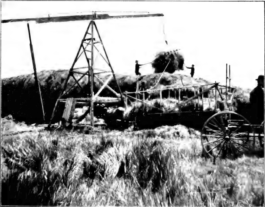
FIG. 2.—DERRICK STACKER, SHOWING DETAILS.
