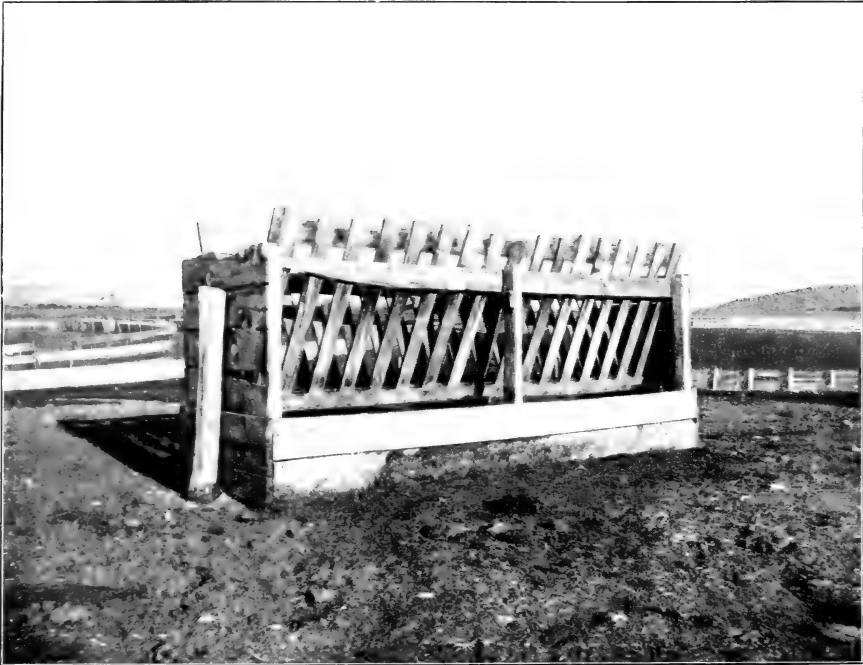
FIG. 1.—LATTICE RACK FOR FEEDING ALFALFA TO CATTLE.
