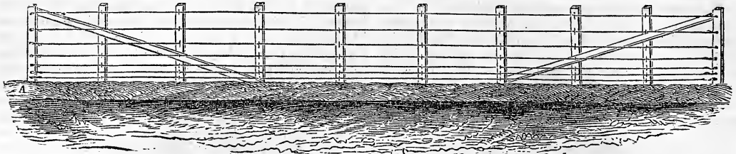
Fig. 1—Section of fence—A. shows the bank, which may be made any required height. The first wire is 4 inches from the ground—the second is 4\frac{1}{2} above that—the third 4\frac{1}{2} —the fourth 6—the fifth 7—the sixth 8, and the seventh 9 inches apart.
