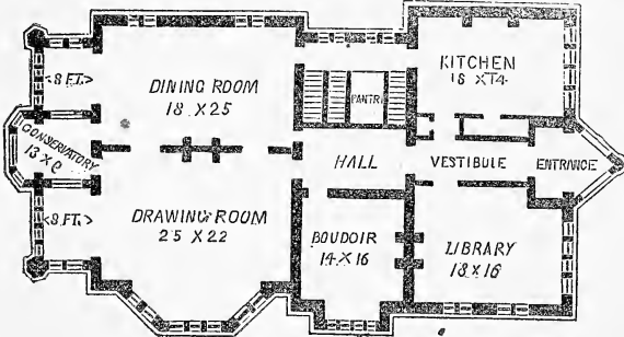
Principal Floor.
