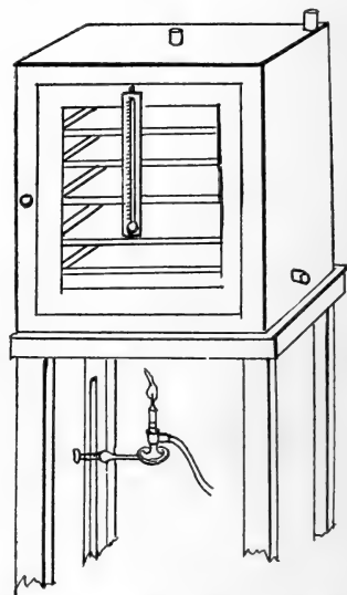
FIG. 7.—Hot water incubator. (Redrawn from Verson and Quajjat.)
