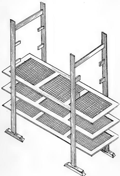
FIG. 5.—Light movable shelves.
