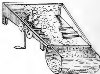
FIG. 11.—Device for removing floss from cocoons. (Redrawn from Nenci.)
