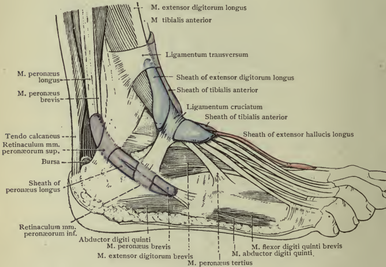
FIG. 158.—Dissection of Leg and Foot showing Mucous Sheath of Tendons.
