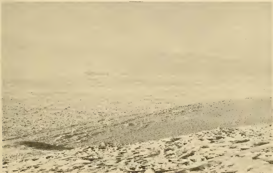
Figure 14. Area between Wales and Diomed Islands illustrating January ice conditions. Fast ice is the dark portion in the lower part of the photograph. All light ice moving north.
