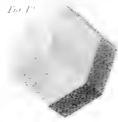
Rhombohedral Dodecahedron. Fig. 12.
