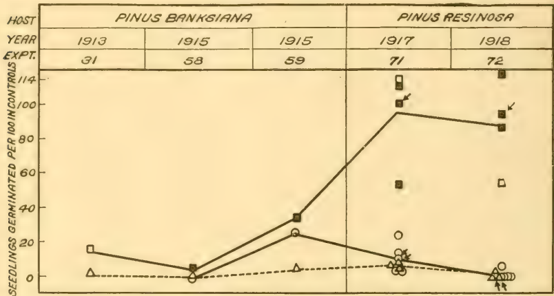
FIG. 10.—Diagram showing the relative activity of different strains of Corticium vagum , as indicated by the number of seedlings appearing in inoculated pots. Explanation of symbols: ○ = Strain 147, from spruce seedlings, Washington, D. C., 1910; ▽ = strain 213, from sugar beet seedlings, Washington, D. C., 1911; ■ = strain 230, from Elacagnus sp., Kansas, 1913; □ = strain 233, from the same lesion as strain 230. Strains reisolated from these, the results of which appear in experiments Nos. 71 and 72, are indicated by the same signs as the original strains used in the inoculations from which they were taken. The original strains in experiments Nos. 71 and 72 are indicated by arrows.
