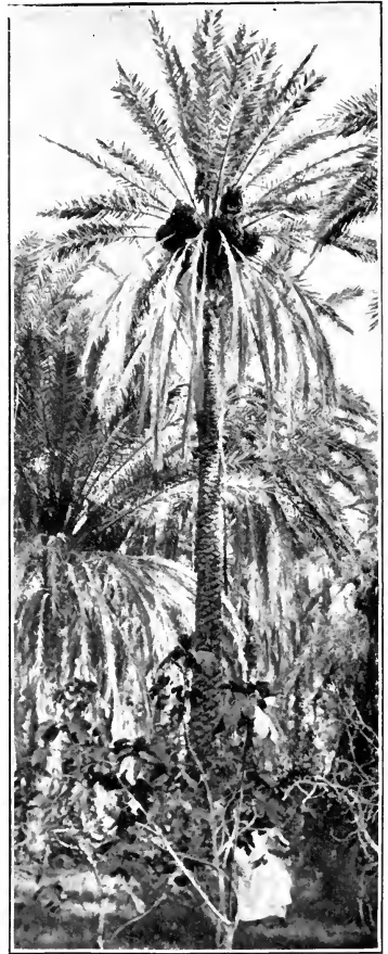
FIG. 2.—LAGOO PALM.
