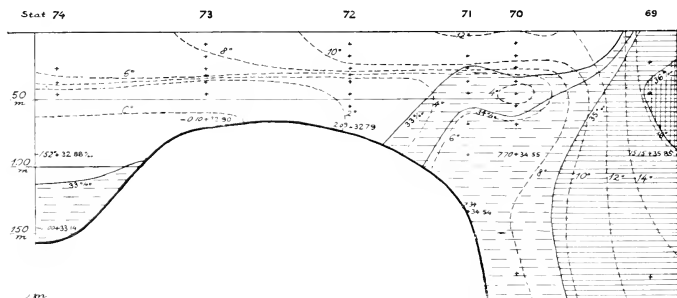
FIG. 95.—HYDROGRAPHICAL SECTION ACROSS THE GREAT NEWFOUNDLAND BANK.
