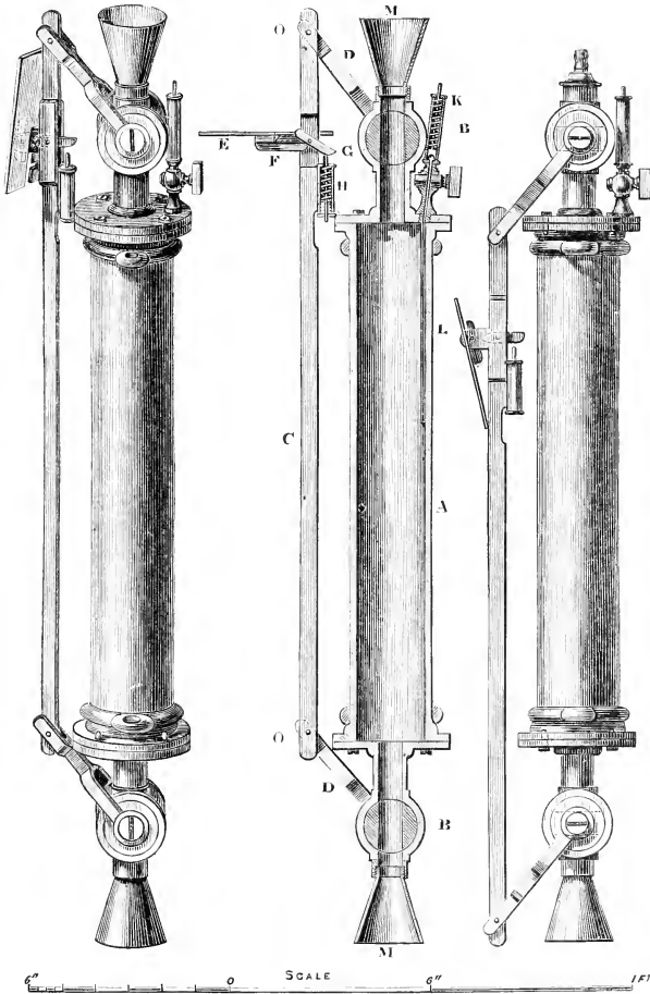
FIG. 161.—BUCHANAN'S STOPCOCK WATER-BOTTLE.
