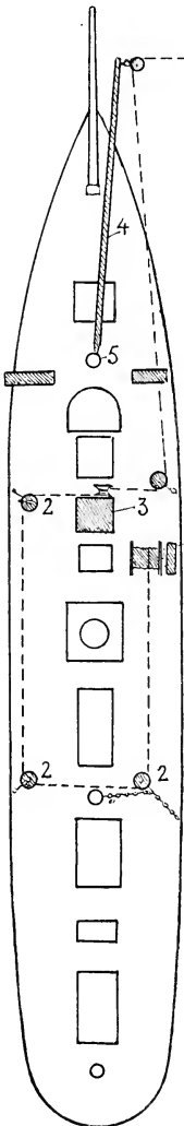
FIG. 9.—DECK ARRANGEMENT OF THE "BLAKE." (From Sigsbee.)
