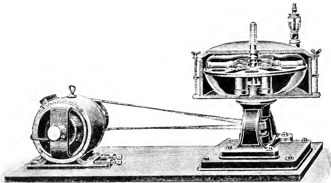
FIG. 35.—CENTRIFUGE DRIVEN BY ELECTRIC MOTOR. (From a catalogue.)
