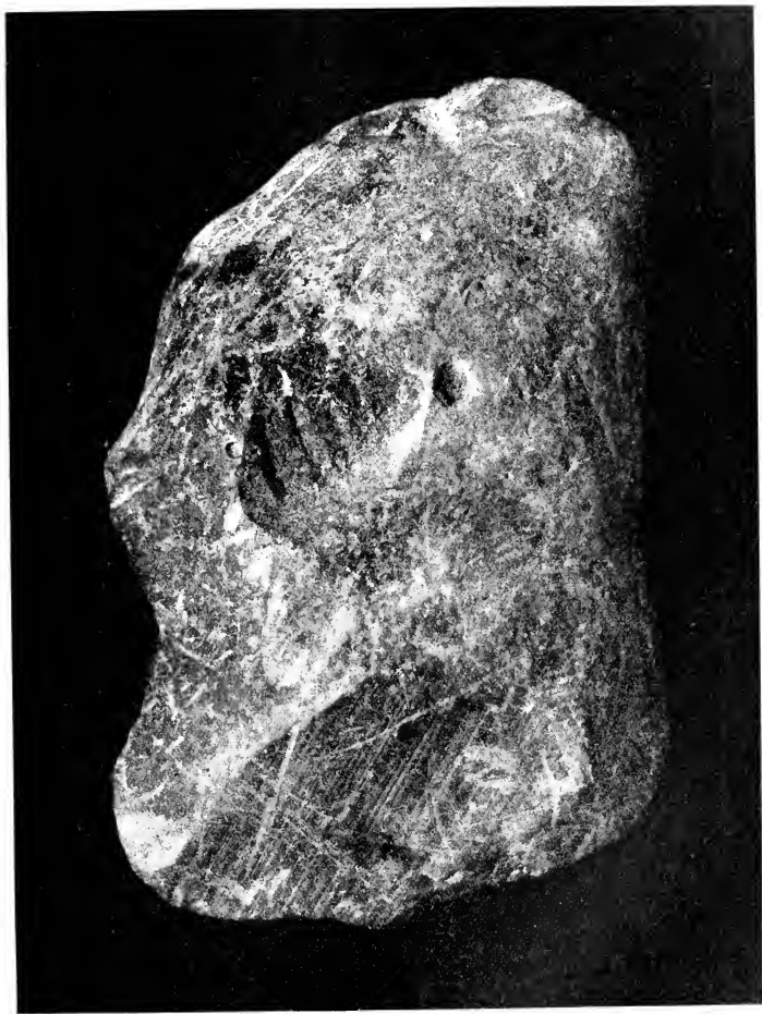
FIG. 145.—GLACIATED STONE FROM "MICHAEL SARS" STATION 95.
