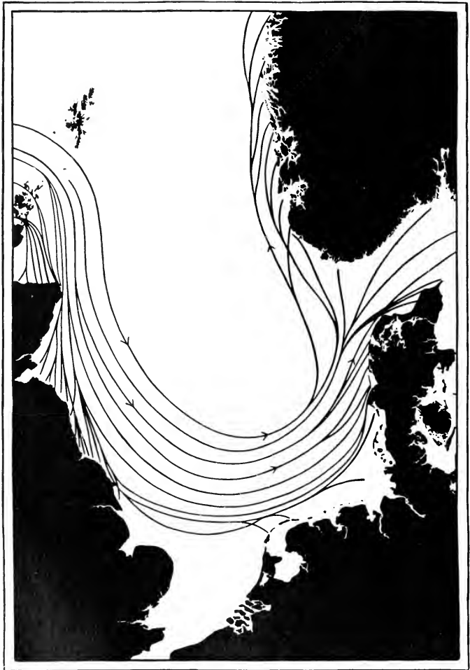
FIG. 176.—RESULTS OF DR. FULTON'S DRIFT-BOTTLE EXPERIMENTS IN THE NORTH SEA.
