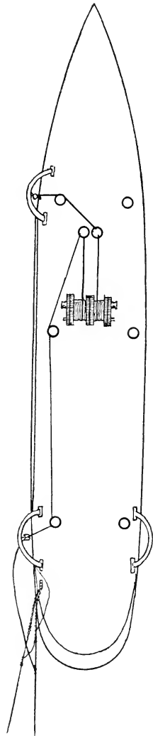
FIG. 25.—DECK ARRANGEMENTS OF A TRAWLER.
