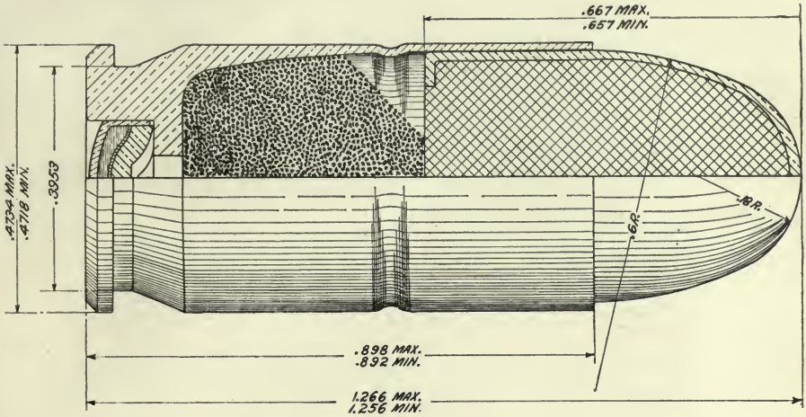
PISTOL BALL CARTRIDGE, CALIBER .45, MODEL OF 1911.
