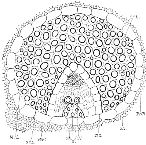
FIG. 2.—Sisal hemp ( Agave rigida var. sisalana ). Transverse section through a fibro-vascular bundle embedded in (PAR) the cellular parenchyma: S.S. starch layer, forming a ring round the sclerenchyma (SCL.), with the fiber cells closely packed together; M.L., middle lamella; B.S., bundle sheath; X., xylem, or wood cells; P.H., phloem, or bast cells. 300.
