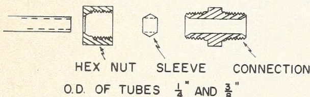
FIGURE 6.—Pressure-tight fitting for refrigeration tubing.
