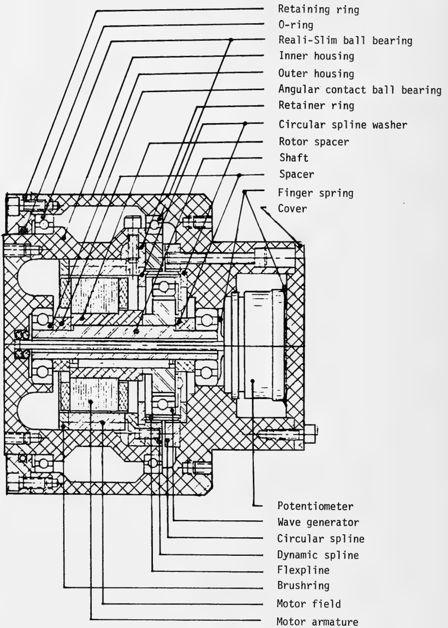
CROSS SECTION OF MOTOR UNIT II
