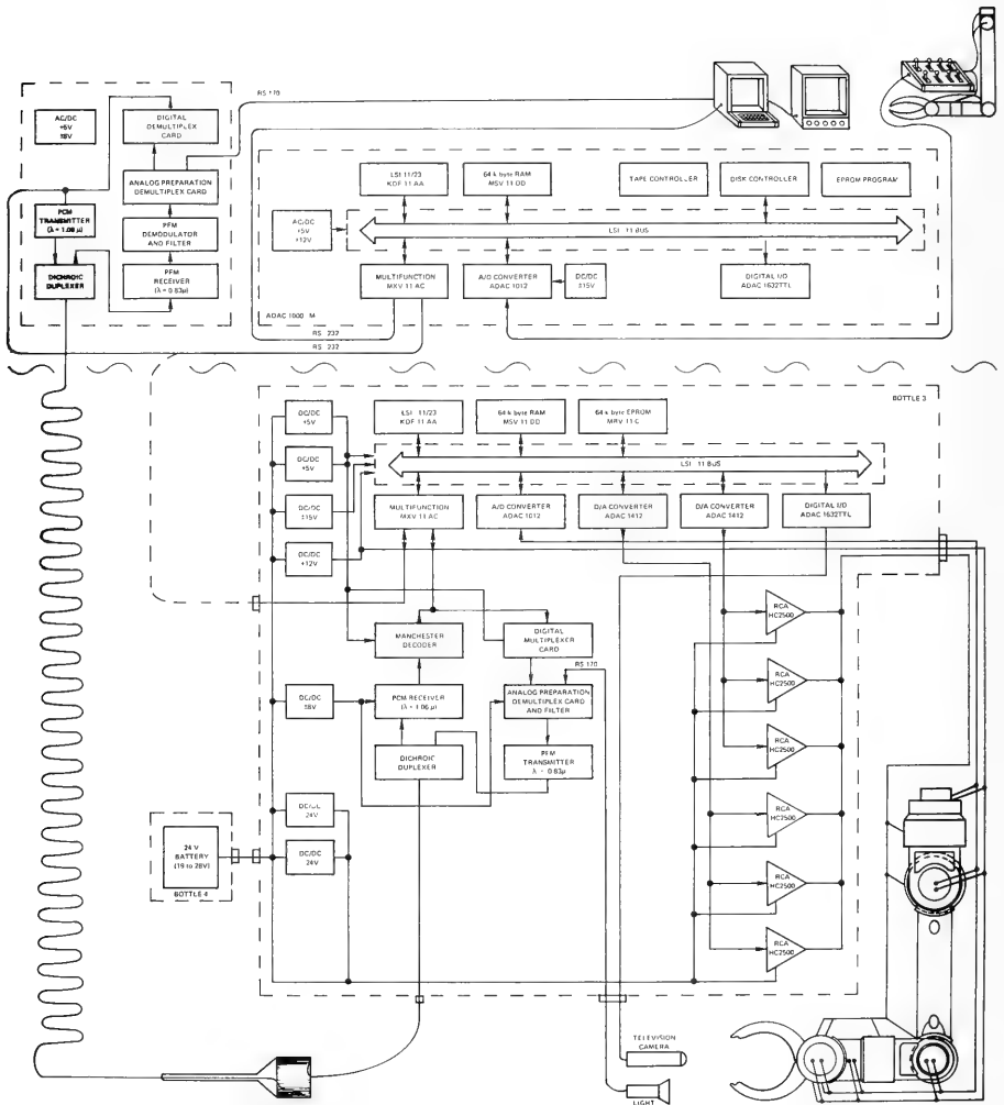
Figure 9. NOSC free-swimmer manipulator supervisory control block diagram.
