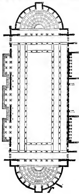
Scaia | | | | | 100 m 100 m (12) * PLAN OF BASILICA ULPIA; see p. 55. (After Canina.)
