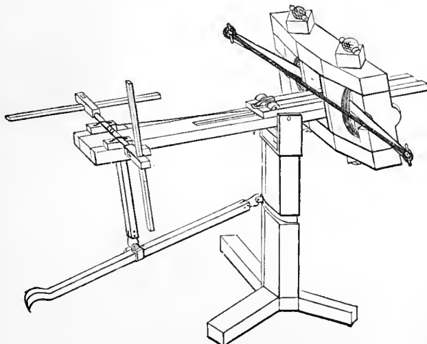
(2) CATAPULT.
