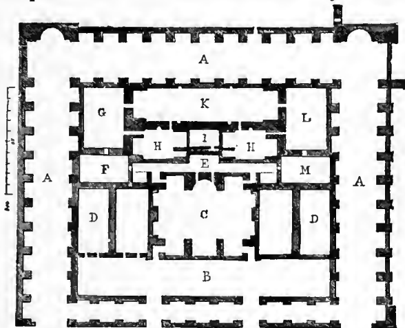
A. Portico. E. Passage. L, M. Warm baths. B. Palaestra. F, G. Cold baths. Near I. Staircase to laconicum. C. Ephēbetōn. H, H'. Hot baths. K. Ball-alley. D. Dressing-rooms.
