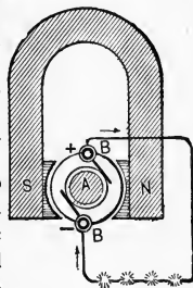
Fig. 361. Magneto-Electric Machine.
