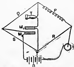
Fig. 81. Hughes' Inductance Bridge.
