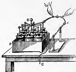
Fig. 40. Leyden Jar Battery.
