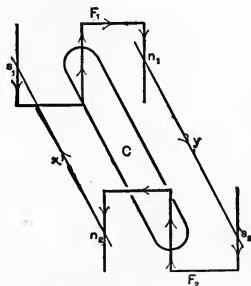
Fig. 390. Eickmeyer's Differential Magnetometer.
