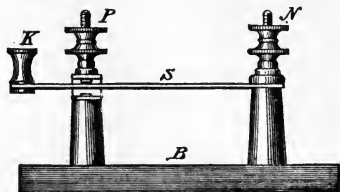
Fig. 329. Short-Circuit Key.
