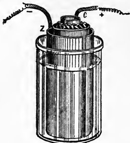
Fig. 106. Daniell's Cell.
