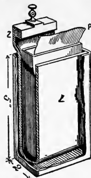
Fig. 110. Grove's Cell.
