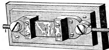
Fig. 263. Safety Fuse.
