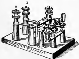
Fig. 328. Reversing Key.
