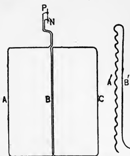
Fig. 182. Rectilinear Equivalent of Sinusoidal Current.
