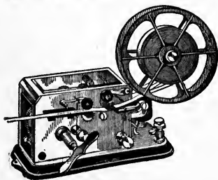
Fig. 473. Ink-Writing Register.
