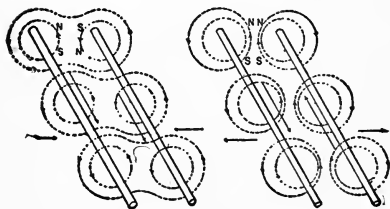
Fig. 222. Mutual Action of Magnetic Fields.
