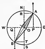
Fig. 174. Magnetic Couple.
