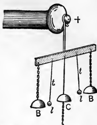
Fig. 121. Electric Chimes.
