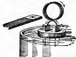
Fig. 38. Floating Cell.
