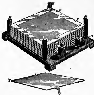
Fig. 169. Air Condenser.
