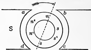
Fig. 292. Horns of Dynamo.
