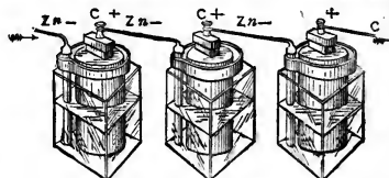
Fig. 133. Voltaic Cells Connected in Series.
