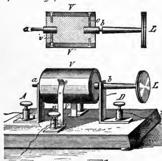
Fig. 160. Ruhmkorff's Commutator
