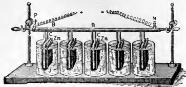
Fig. 42. Plunge Battery.
