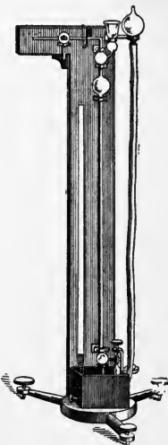
Fig. 454. Geissler's Mercurial Air Pump.
