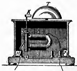
Fig. 8. Automatic Make-and-Break.
