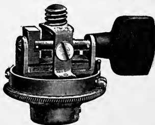
Fig. 522. Lamp-Socket Switch.
