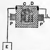
Fig. 27. Counter-Electromotive Force Lightning Arrester.
