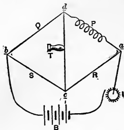
Fig. 80. Inductance Bridge.
