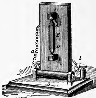
Fig. 397. Microphone.
