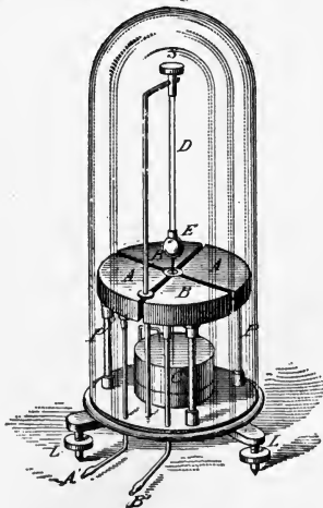
Fig. 234. Quadrant Electrometer.
