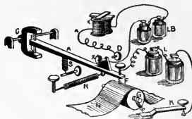
Fig. 399. Electro-Motograph.
