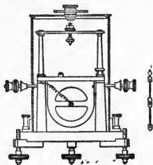
Fig. 270. Nalder's Galvanometer.
