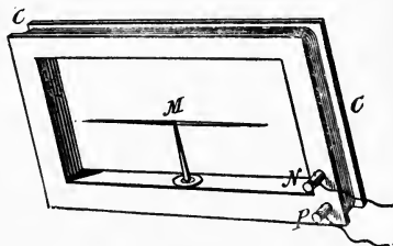
Fig. 266. Schweigger's Multiplier.
