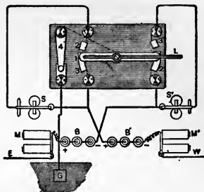
Fig. 484. Wood's Button Repeater.
