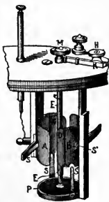
Fig. 486. The Replenisher.
