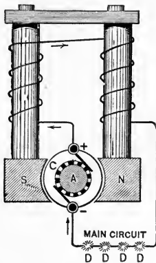
Fig. 354. Series Dynamo.
