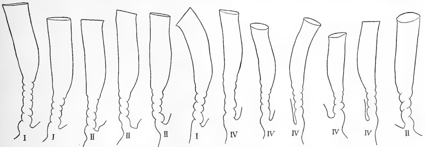
Fig. 18. Lafoëa gracillima (ALDER) forma elegantula . Vergr. \times 52 . Hydrothekenvariation. I Station 15. II Station 32. IV (Original exemplar der Lafoëa elegantula BROCH, 28) 74° 7' n. Br., 19° 4' ö. L., 90 m Tiefe.
