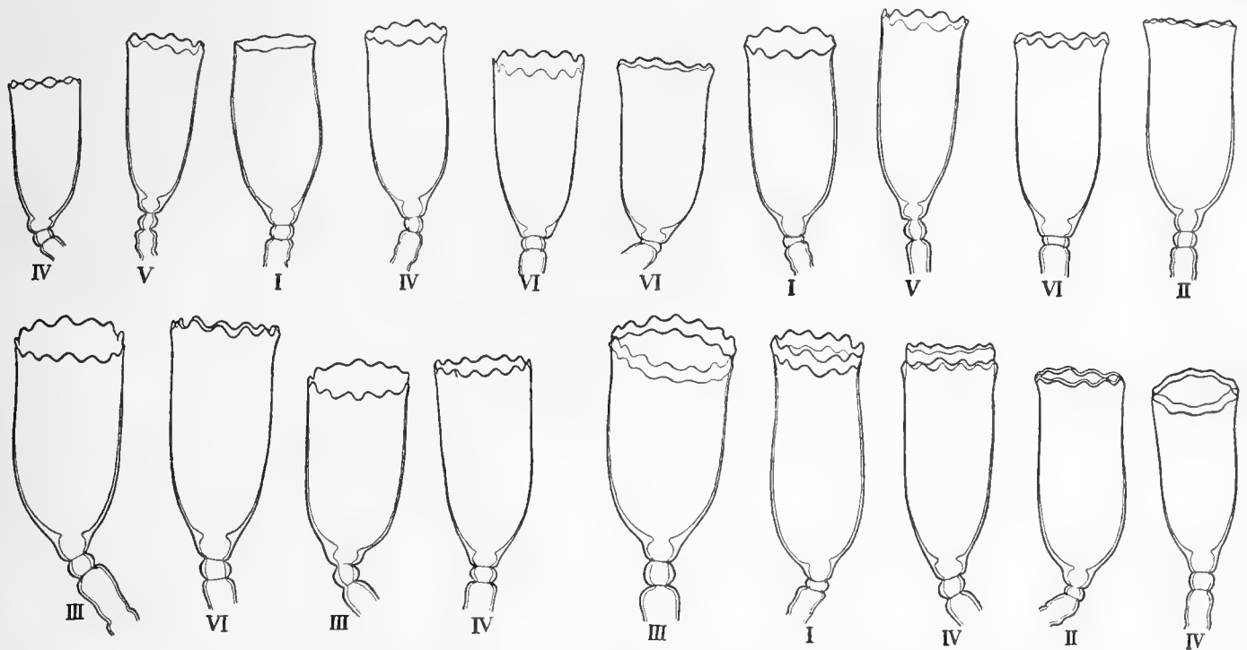
Fig. 39. Campanularia volubilis (LIN.). Vergr. \times 52 . Hydrothekenvariation, I Station 15. II Station 15. III Station 32. IV Station 51. V Station 56. VI Station 59.
