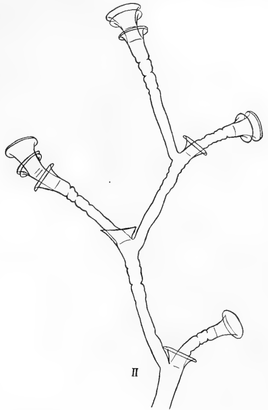
Fig. 13. Halecium sp. ( minutum BROCH aff.). Vergr. \times 36 . Station 56.
