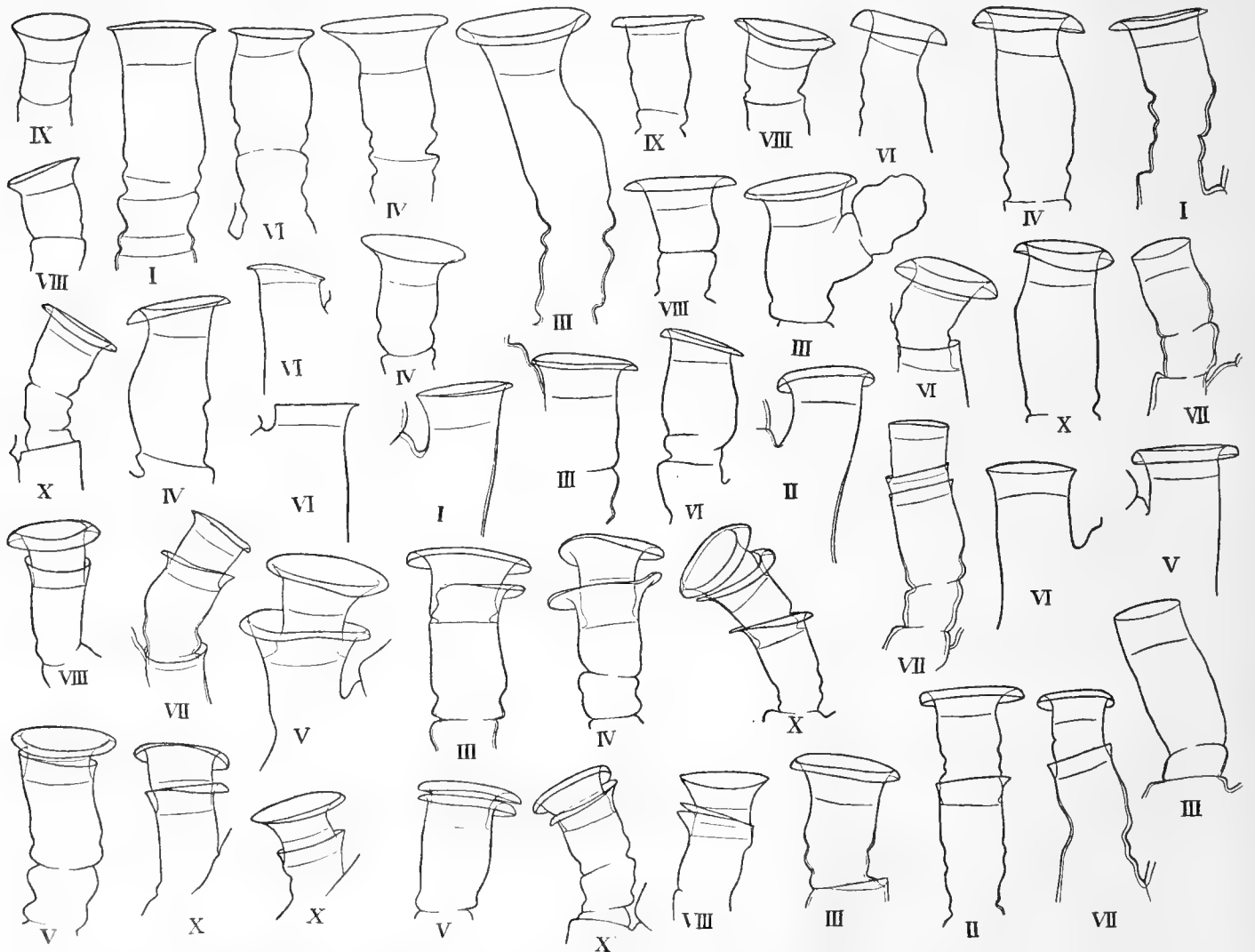
Fig. 7. Halecium labrosum ALDER. Vergr. \times 52 . Hydrothekenvariation. I Station 15. II Station 25, ♀. III Station 32, ♀. IV Station 32, ♀. V Station 37, ♀. VI Station 51, ♀. VII Station 56, ♀. VIII Station 56, ♀. IX Station 56, ♂. X Station 59, ♂.
