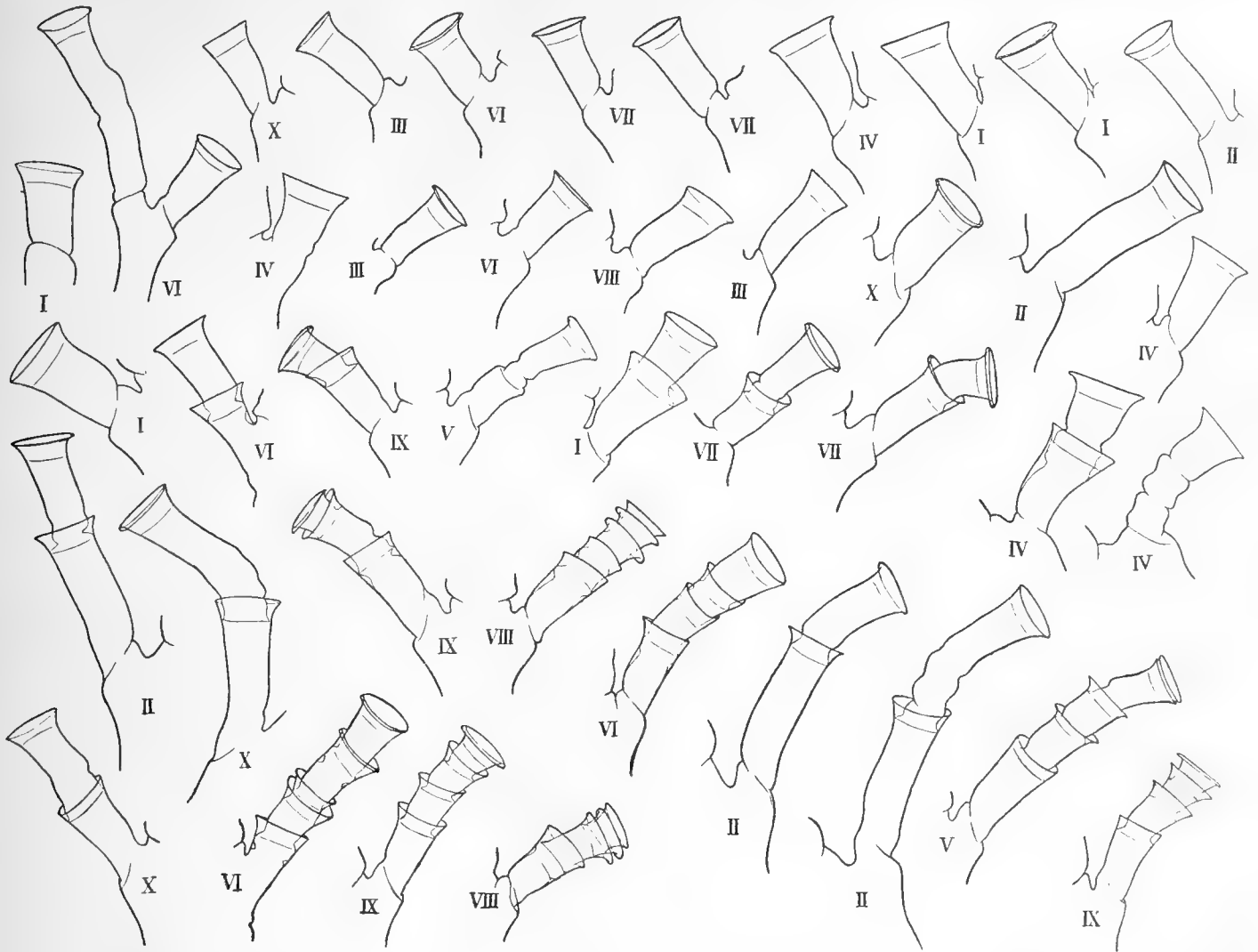
Fig. 6. Halecium 2 muricatum (ELLIS u. SOLANDER). Vergr. \times 52 . Hydrothekenvariation. I Station 2. II Station 27*. III Station 33*. IV Station 45*. V Station 56*. VI Station 59*. VII Station 59. VIII Station 59. IX 62° 16' n. Br. 6° 6' w. L. 110 m Tiefe. X Mittlere Nordsee (57° 8' n. Br. 2° 11' ö. L. 90 m Tiefe) [* mit Gonangien].
