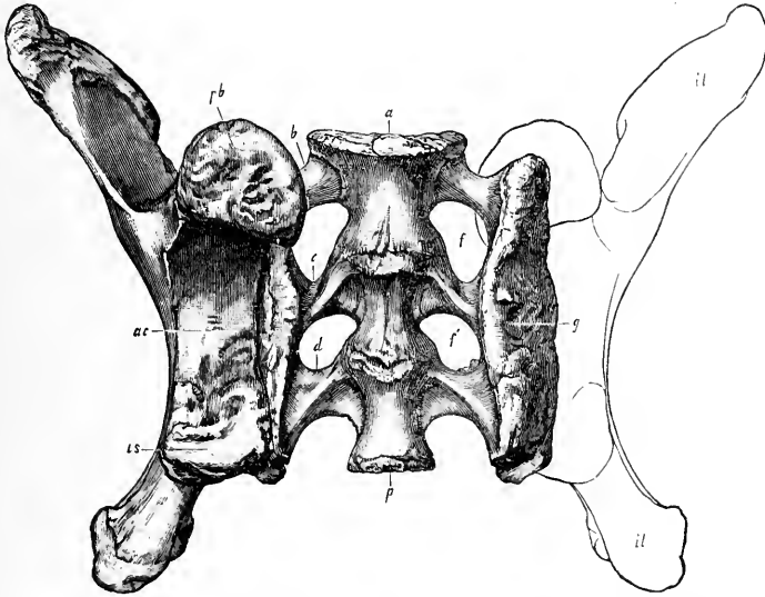
FIG. 10. Sacrum and ilium of Diplodocus longus Marsh; seen from below. With anterior and posterior ends of sacrum reversed. pb , pubic process; is , ischiae process; ac , acetabulum; b , c , d , sacral ribs; f , f' , foramina. One tenth natural size. After Marsh.
