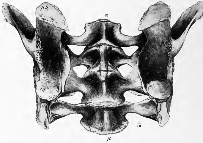
FIG. 9. Inferior view of sacrum and ilia of Diplodocus carnegii (No. 94), one tenth natural size; pb , pubic peduncle; is , ischia peduncle; a , anterior end; p , posterior end.
