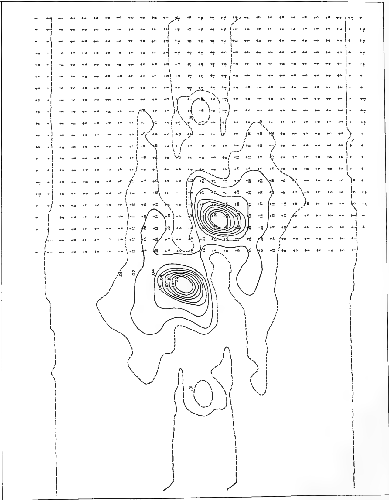
FIG. 119 DIRECTIONAL SPECTRUM FOR DATA SET NUMBER 2
