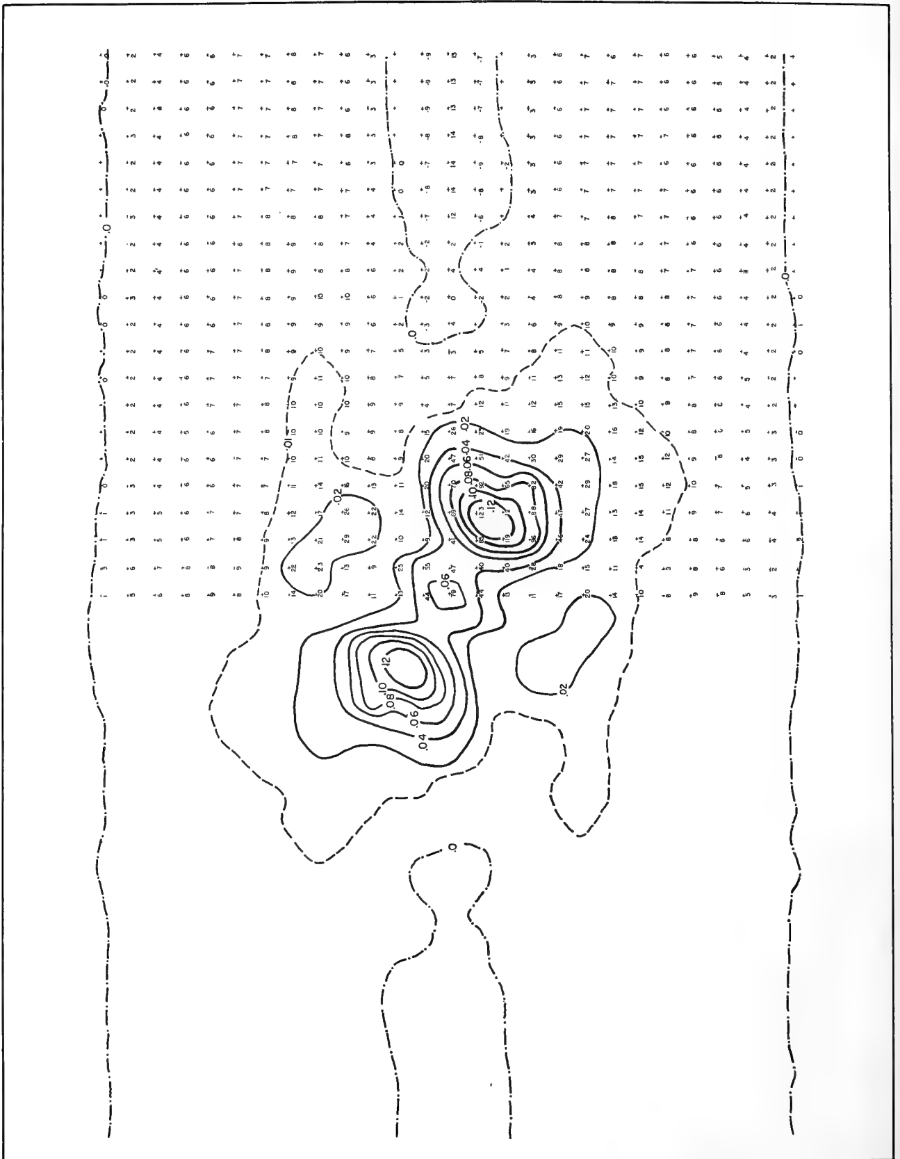
FIG. 11.11 \frac{u_x + u_y}{2}
