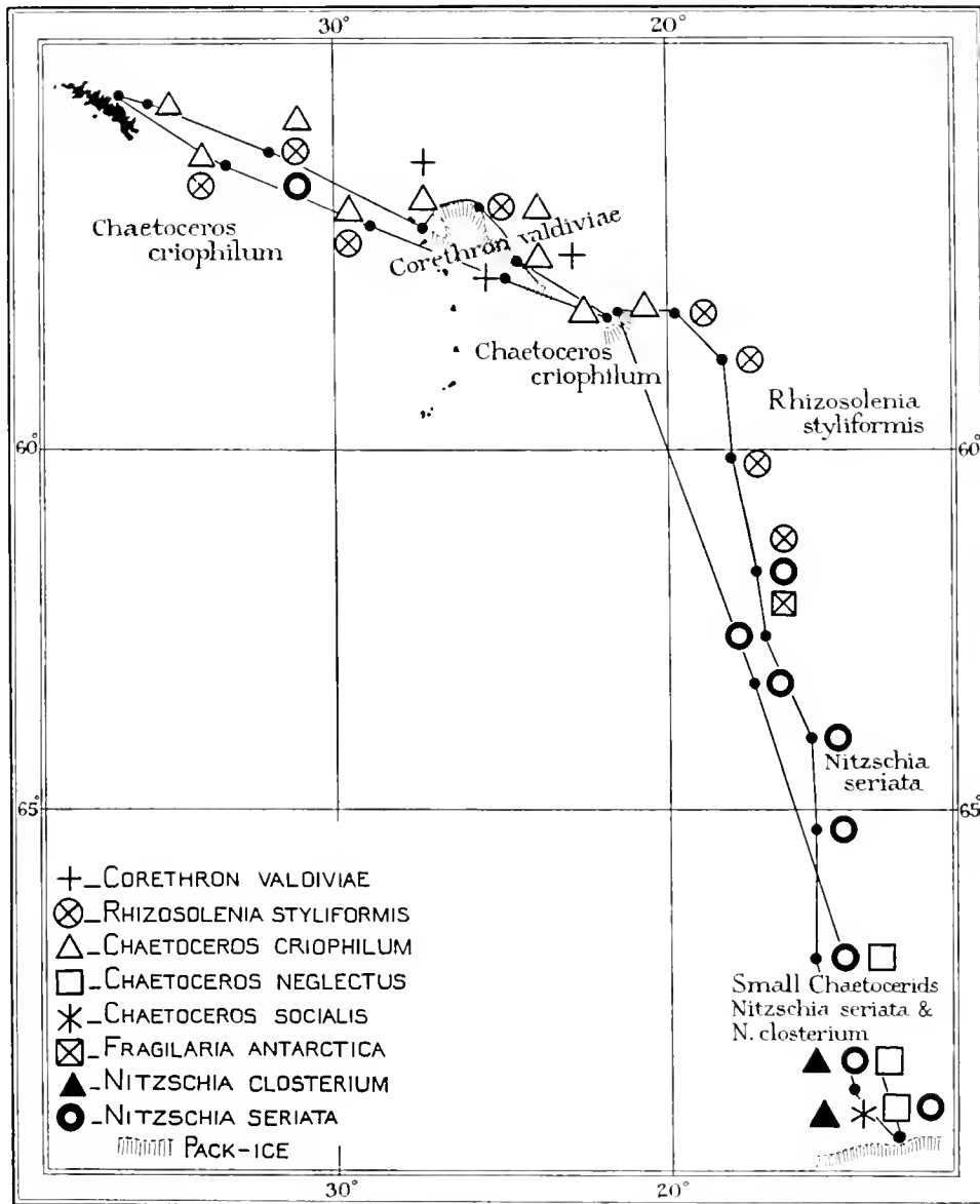
Fig. 48. Distribution of the principal phytoplankton species in the eastern Weddell Sea, January-February 1931.
