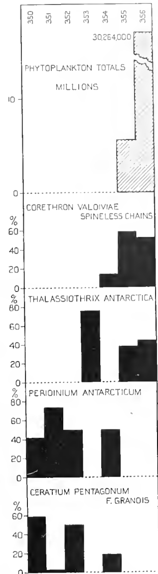
Fig. 11. Diagram showing the percentages of the principal species in the catches on the Vakop Line, South Georgia survey, January–February 1930.
