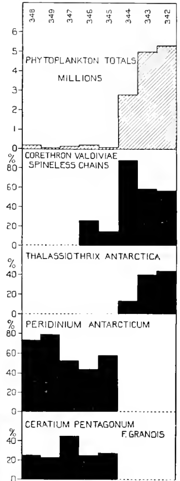
Fig. 10. Diagram showing the percentages of the principal species in the catches on the Cooper Island Line, South Georgia survey, January-February 1930.
