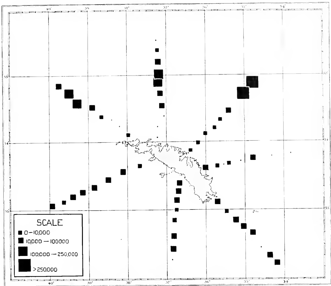
Fig. 16. The distribution of Ceratium pentagonum f. grandis , South Georgia survey, January-February 1930.
