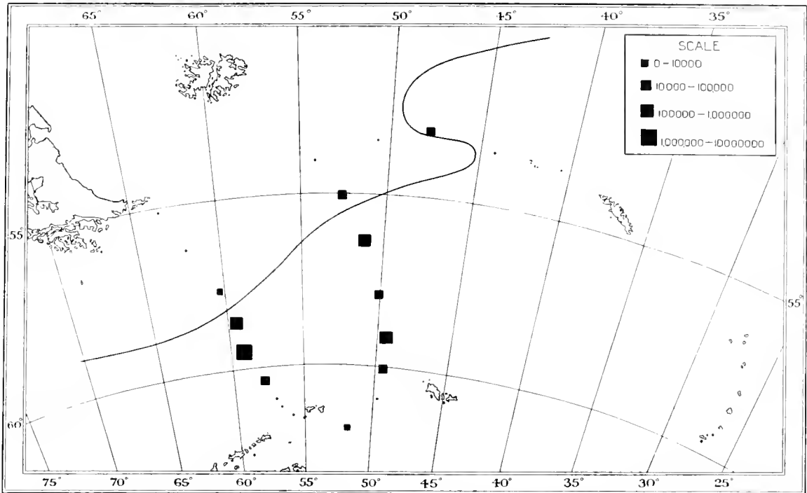
Fig. 44. The distribution of Fragilaria antarctica in the Scotia Sea, February-March 1931.
