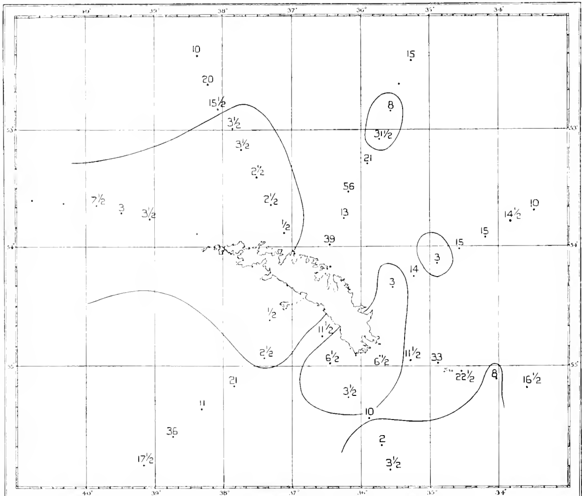
Fig. 22. The distribution of Chaetoceros criophilum , South Georgia survey, November 1930. 1 = one million.
