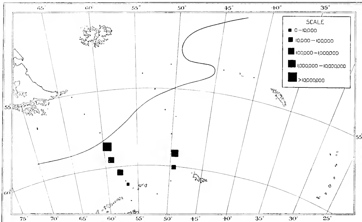
Fig. 42. The distribution of Chaetoceros neglectus in the Scotia Sea, February–March 1931.
