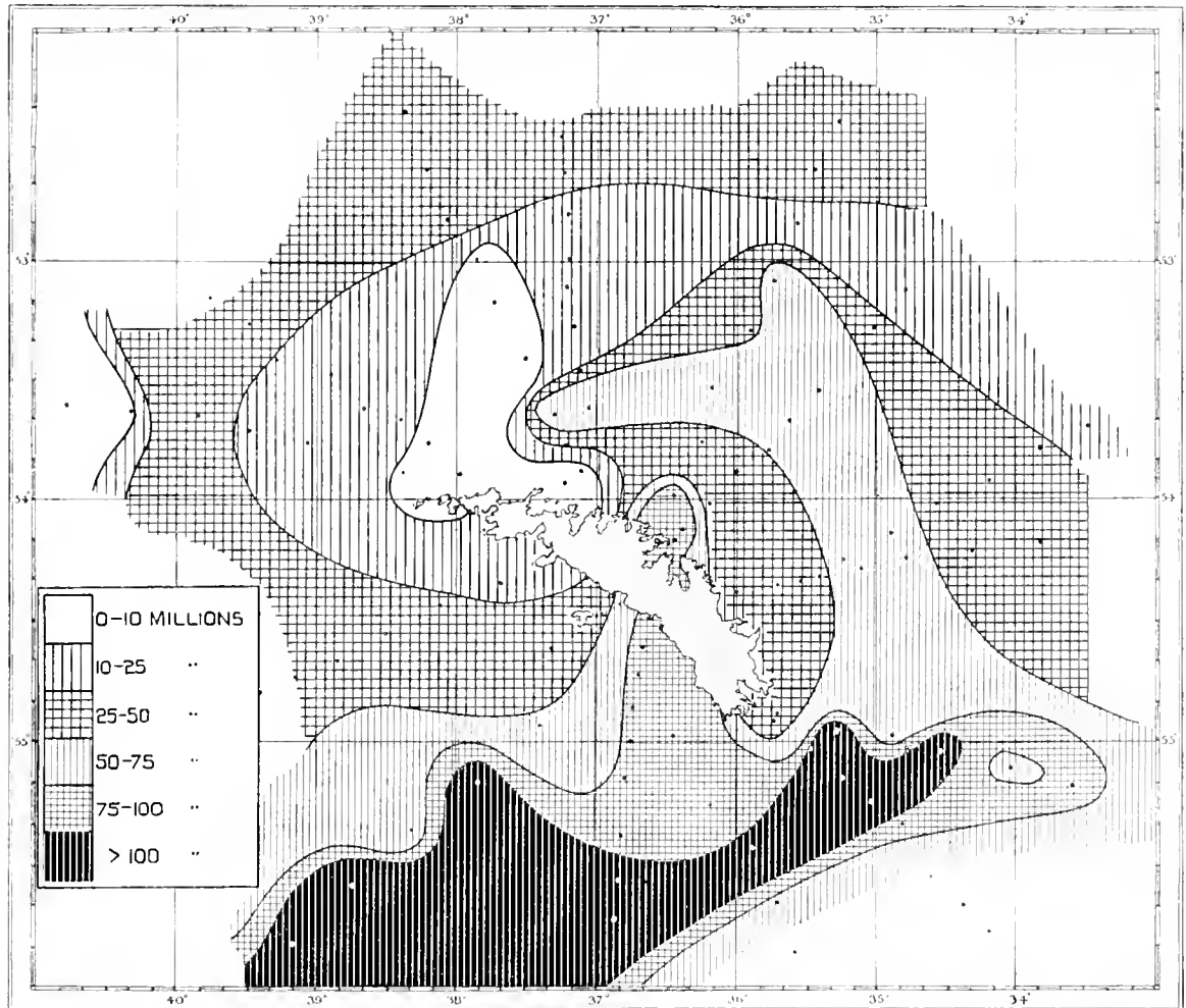
Fig. 18. General distribution of Diatomales (totals per 100-0 m. haul), South Georgia survey, November 1930. This chart is based on catches made at the positions indicated in Fig. 19.
