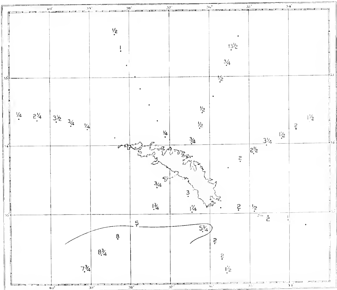
Fig. 26. The distribution of Nitzschia seriata , South Georgia survey, November 1930. 1 = one million.
