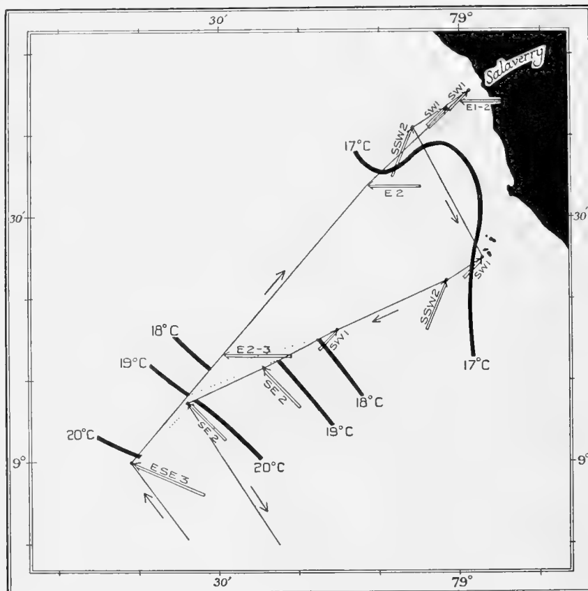
Fig. 35. Changes in wind and in the distribution of surface isotherms off the Gunaípe Islands in the period July 9-11, 1931. Symbols as in Fig. 28. Station positions may be identified by collation with Fig. 13. The dotted lines show the shift of the isotherms of 18, 19 and 20^{\circ}\text{C} . (see Table IV).
