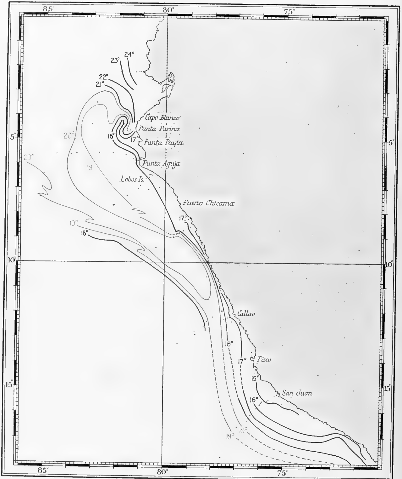
Fig. 16. Distribution of surface isotherms off Peru, June to August, 1931. An alternative construction is placed on the same data in Fig. 63.
