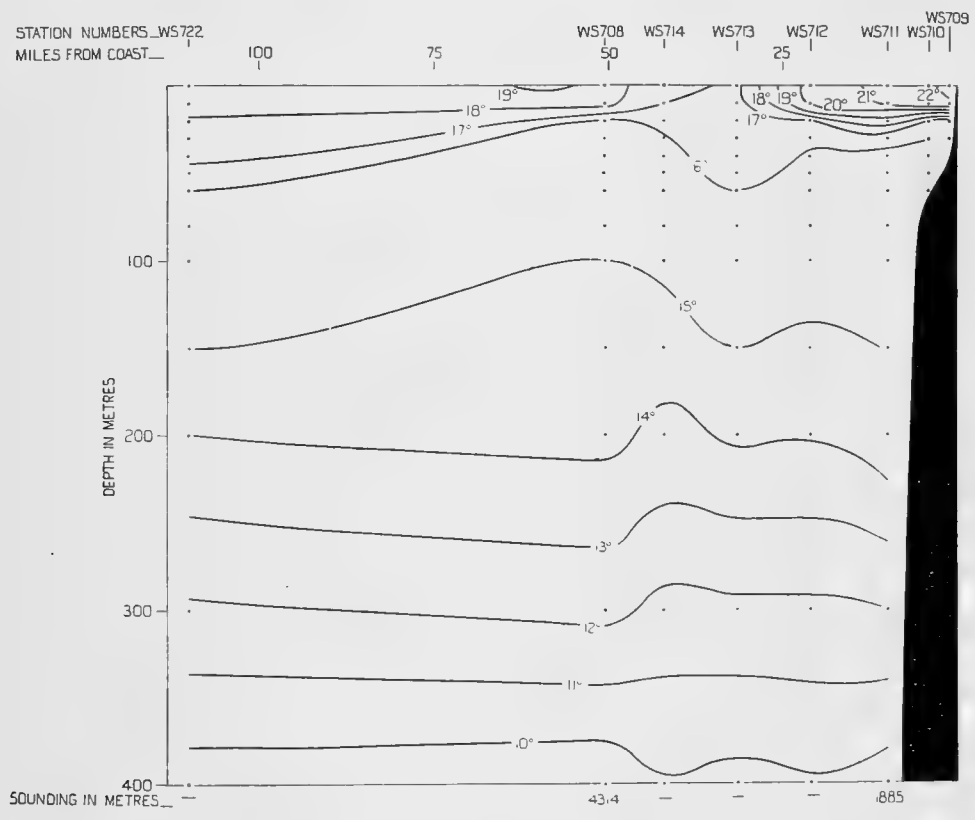
Fig. 41. Distribution of temperature ( ^{\circ} C.). Section off Capo Blanco, July 24–26. The positions of the sections on this page are shown in Figs. 2, 70 and 71; the corresponding salinity sections, on pp. 169 and 168.
