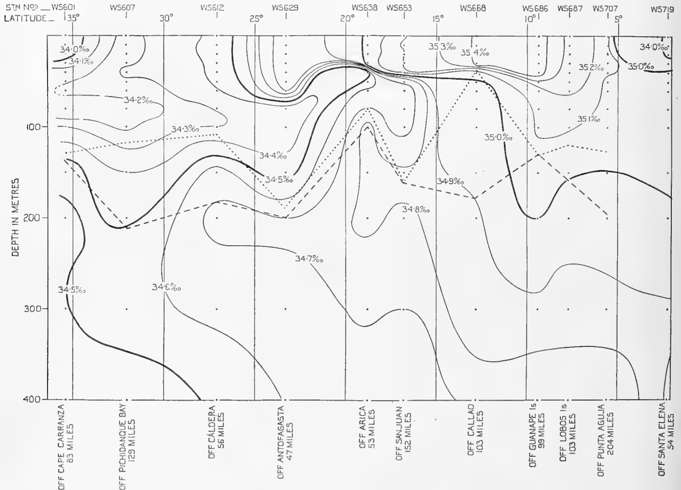
Fig. 42. Section illustrating the distribution of salinity in the upper 400 metres along the path of the current. The section runs roughly parallel to the coast and is situated at a mean distance of about 100 miles from it. The dotted line indicates the value of the surface salinity at the inshore station corresponding to each of the stations plotted; and the broken line indicates the maximum depth apparently affected by upwelling at each of these localities.
