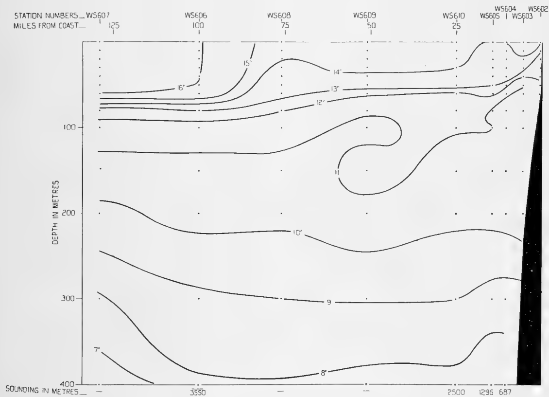
Fig. 21. Distribution of temperature (°C). Section off Pichidanque Bay, May 28-30.
