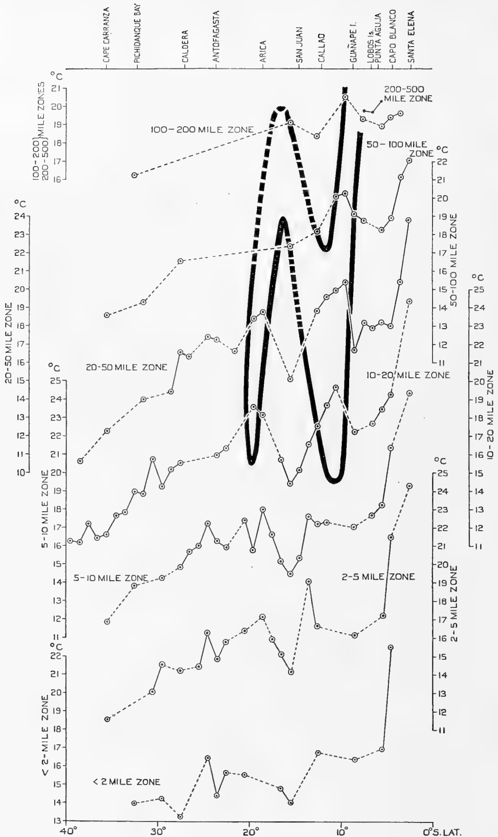
Fig. 34. Curves illustrating the mean surface temperature along the path of the current. Each curve represents the temperature of a zone at a given distance from the shore, the data within it being averaged separately for each degree of latitude (Appendix VI). The curves are broken where data are wanting. Regions influenced by an inflow of warm oceanic water ( vide warm wedge in text) are indicated by a heavy line.
