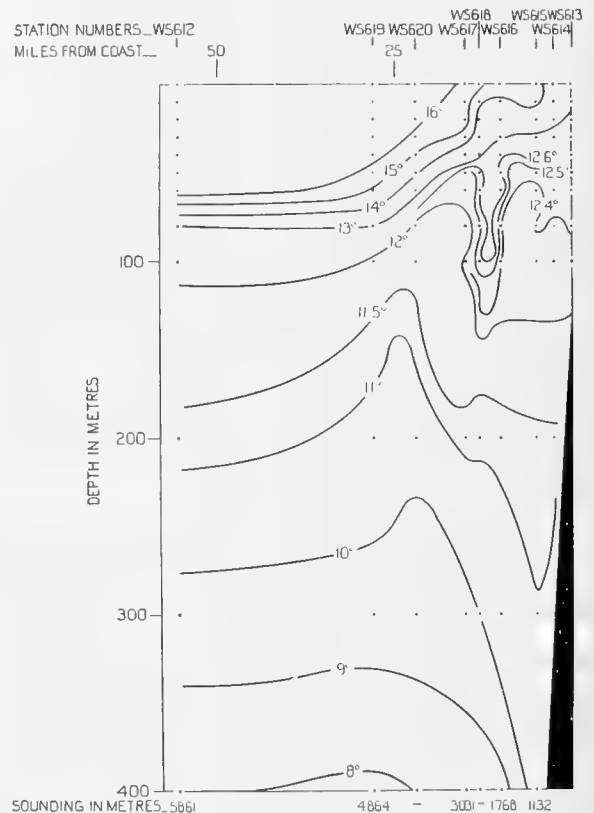
Fig. 23. Distribution of temperature ( ^{\circ}\text{C} .). Section off Caldera, June 4-6.
