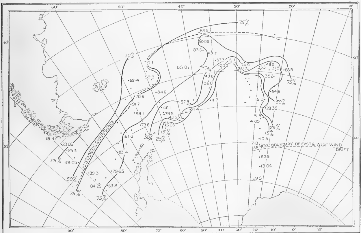
Fig. 9. Percentage distribution of Rhincalanus gigas in the Falkland Sector of the Antarctic, mid-November 1931 to mid-January 1932. (1-m. nets, 250-100 m. approx. and 100-0 m. approx.) Numbers represent percentage of R. gigas in the total copepod catch in the upper and lower hauls together.
