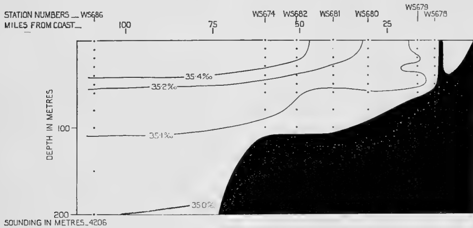
Fig. 48. Distribution of salinity. Section off the Guañape Islands, July 10-11. The position of this section is shown in Figs. 2 and 13.
