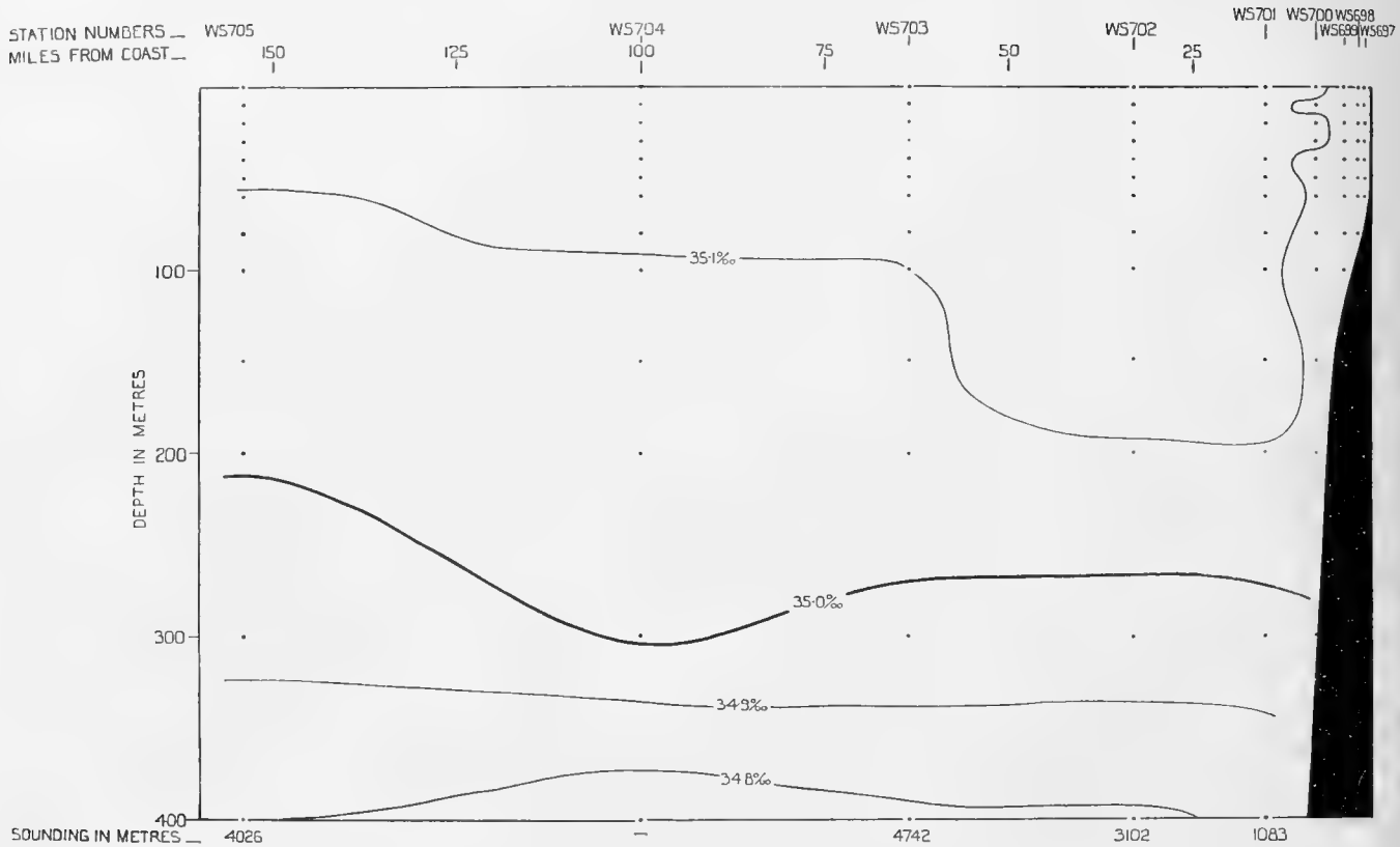
Fig. 46. Distribution of salinity. Section off Punta Aguja, July 21-23. The position of this section is shown in Figs. 2 and 12; the corresponding temperature section, in Fig. 36.
