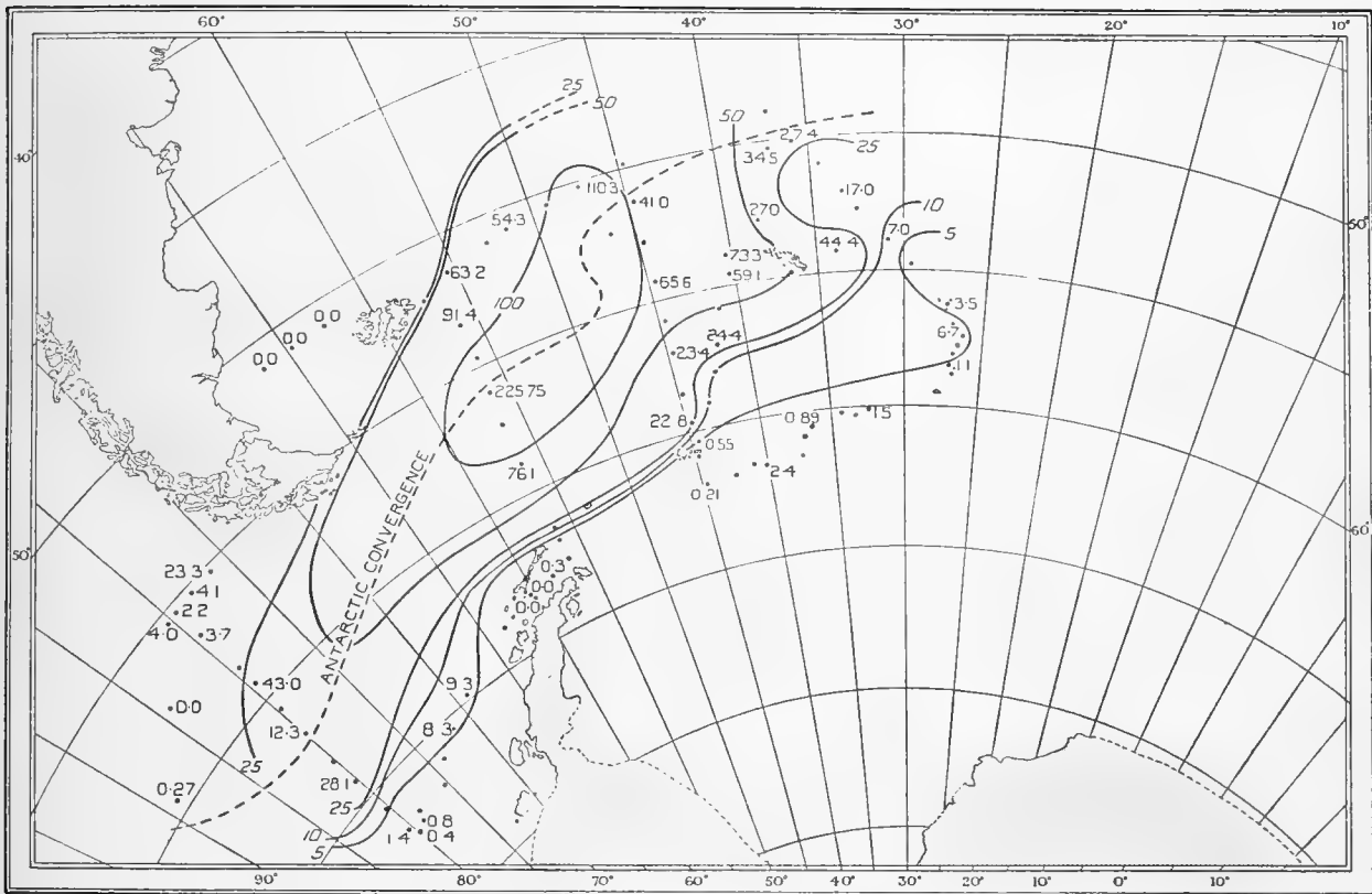
Fig. 14. Horizontal distribution of Rhincalanus gigas in the Falkland Sector of the Antarctic, October to December 1932. (1-m. nets, 250-100 m. approx., 100-0 m. approx., both hauls combined.) Numbers represent hundreds of individuals.
