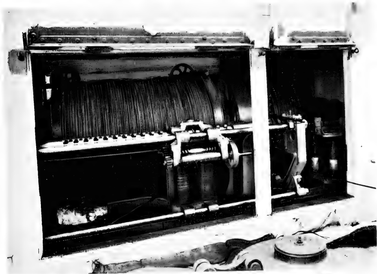
RRS 'DISCOVERY II'. AFTER-DECK MACHINES
