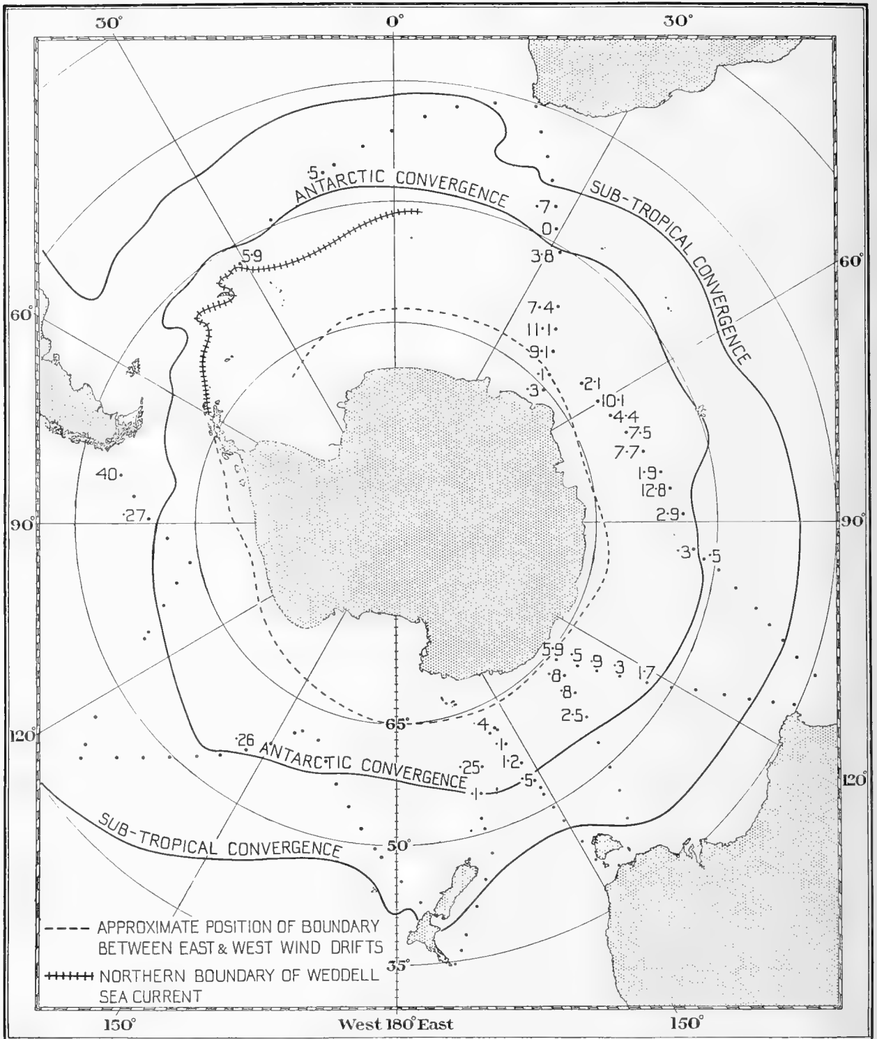
Fig. 11. Horizontal distribution of Rhinocalanus gigas around the Antarctic Continent, winter months, February to October 1932. (1-m. nets 250-100 m. approx., 100-0 m. approx., both hauls combined.) Numbers represent hundreds of individuals.
