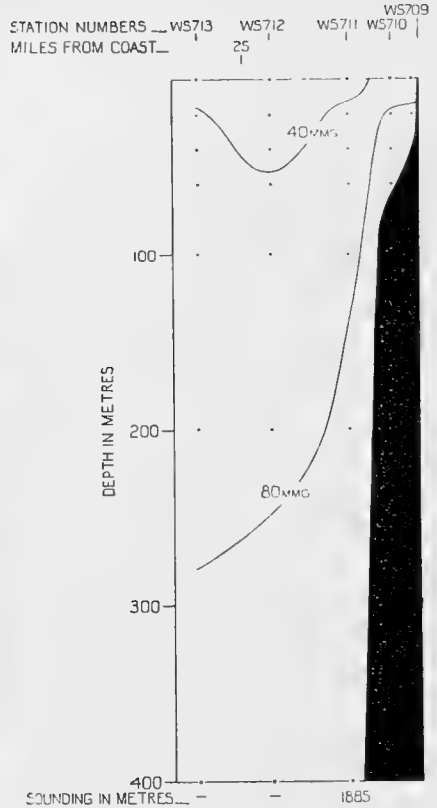
Fig. 40. Distribution of phosphate (per m.^3 ). Section off Capo Blanco, July 24–26.
