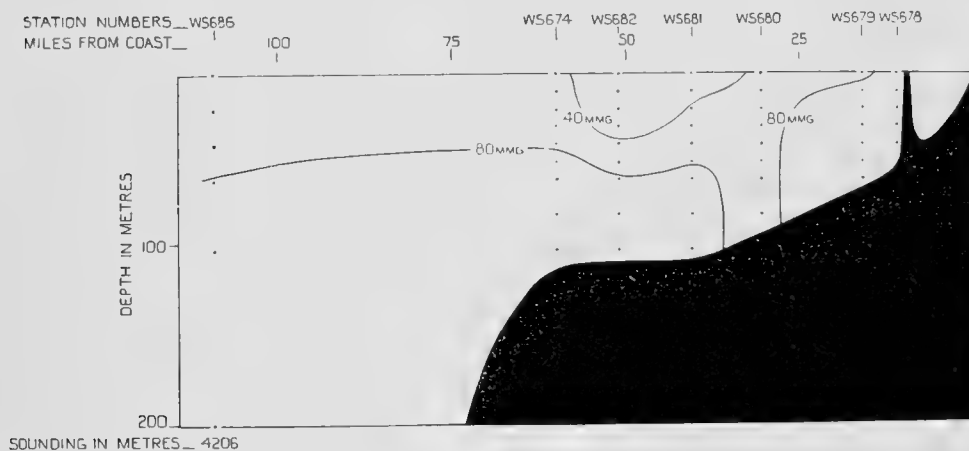
Fig. 61. Distribution of phosphate (per m. 3 ). Section off the Guañape Islands, July 10-11.
