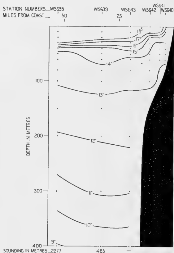
Fig. 31. Distribution of temperature (° C.). Section off Arica, June 19-20. The position of this section is shown in Figs. 3 and 11; the corresponding salinity section, in Fig. 43.
