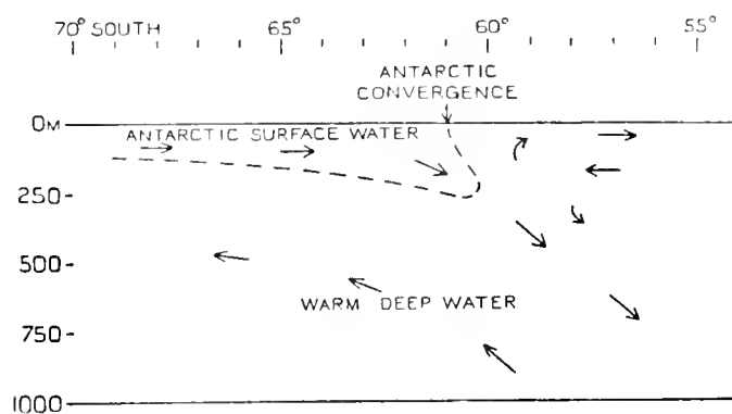
Fig. 2. Water movements in 80° W.
