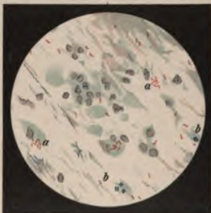
Fig. 158.—Tubercle Bacilli and Micrococcus Tetragenus (sputum). Gabbet's stain, Leitz ocular I, oil immersion \frac{1}{10} . (a) tubercle bacilli; (b) micrococcus tetragenus. (Lenhartz-Brooks).
