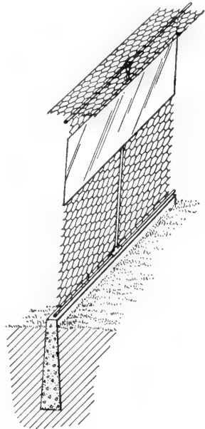
FIG. 20.—Section of a fence containing a smooth zone to protect foxes from injury from falling. Concrete foundation and iron posts.
