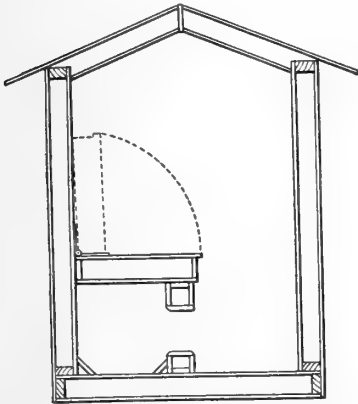
FIG. 8.—Vertical cross section of double-walled den.
