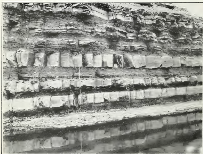
FIG. 2.—SHALES HAVING NEARLY HORIZONTAL LAYERS WHICH HAVE BEEN CUT BY CLEAVAGE PLANES CAUSED BY GREAT PRESSURE.
