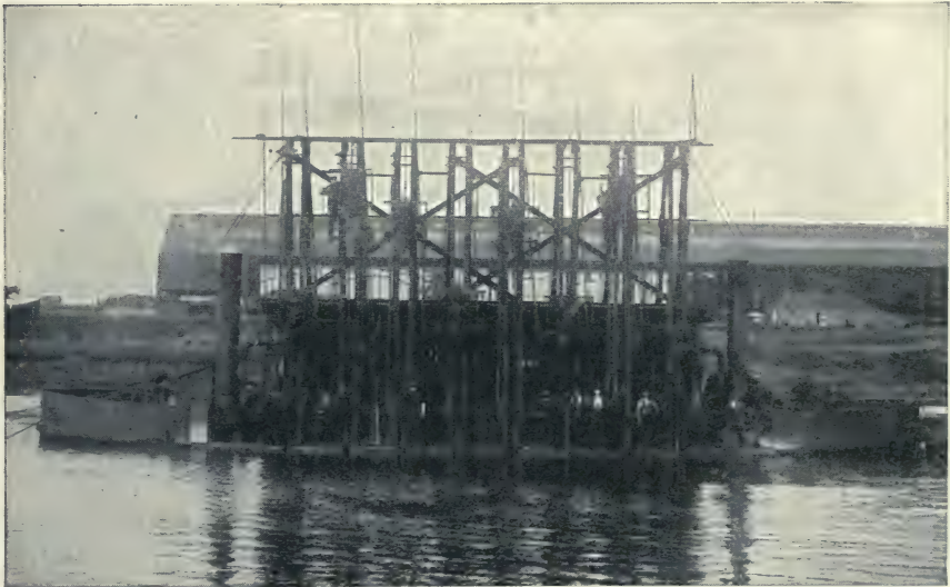
FIG. 5.—Saunderson's Machine for Subaqueous Rock Excavation.
