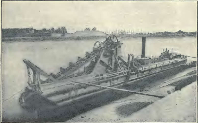
FIG. 20.—Dredge on the Rhone River Propelled by Sprocket Wheel.
