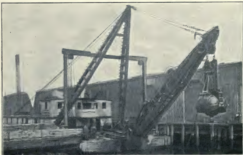
FIG. 58.—Dredge "Champion."
