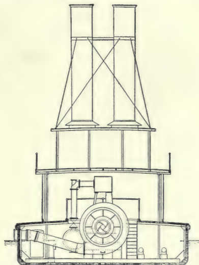
FIG. 38.—Cross-section of the Dredge "King Edward VII."
