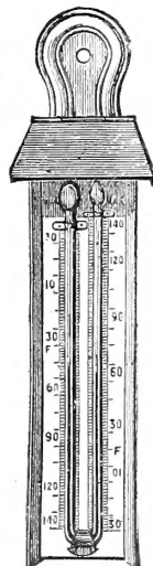
SELF-REGISTERING THERMOMETER.
