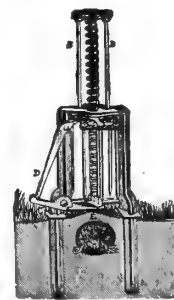
OLMSTED MOLE TRAP.
