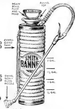
4-Gallon Tank Double Bottom—Double Strength Compressed Air Sprayer
