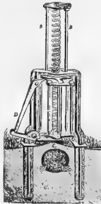
OLMSTED MOLE TRAP
