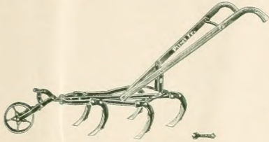
No. 100. Planet Jr. Plain Cultivator
