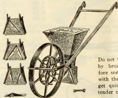
No. 20D Planet Jr. Fertilizer Distributer
