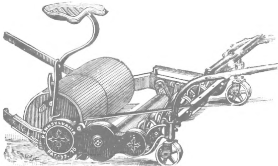
PENNSYLVANIA HORSE MOWER—OLD STYLE
